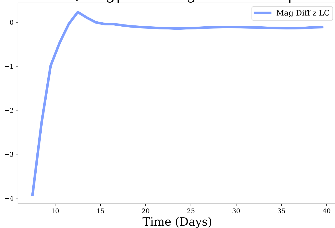
z-band, Avg|Max Mag Diff: -0.31 | 3.92
