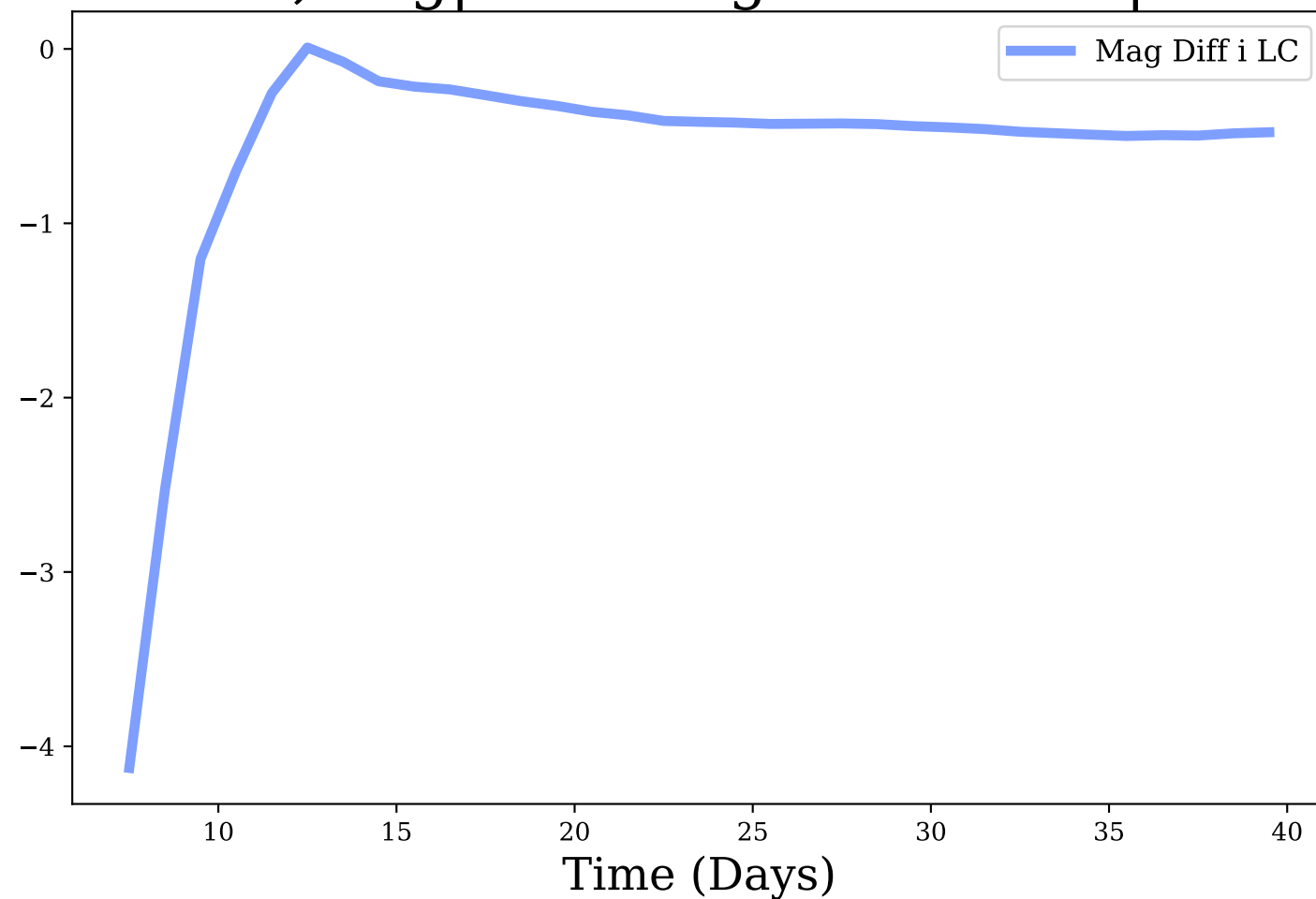
i-band, Avg|Max Mag Diff: -0.59 | 4.12
