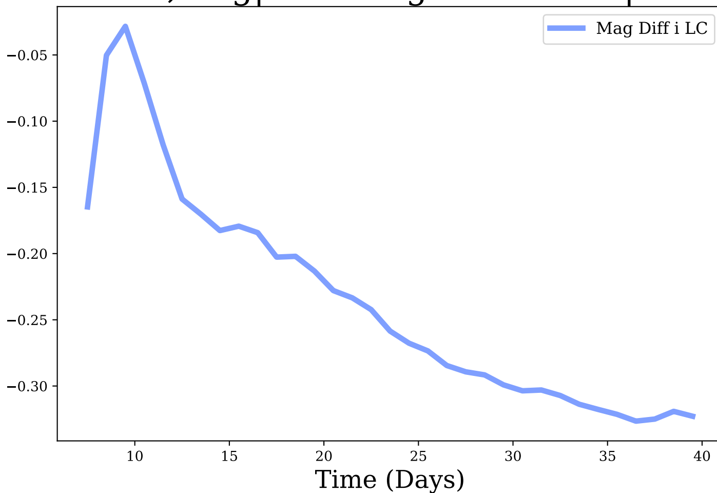
i-band, Avg|Max Mag Diff: -0.23 | 0.33
