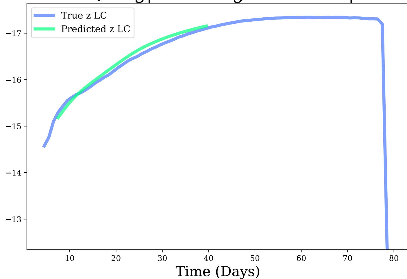
z-band, Avg|Max Mag Diff: 0.09 | 0.13
