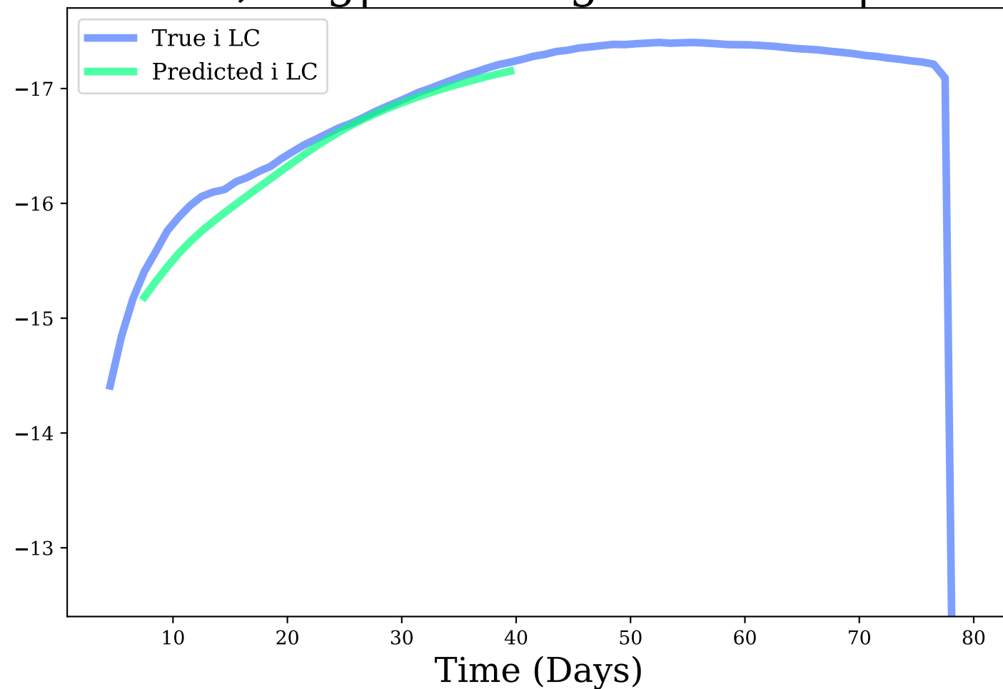
i-band, Avg|Max Mag Diff: 0.12 | 0.32
