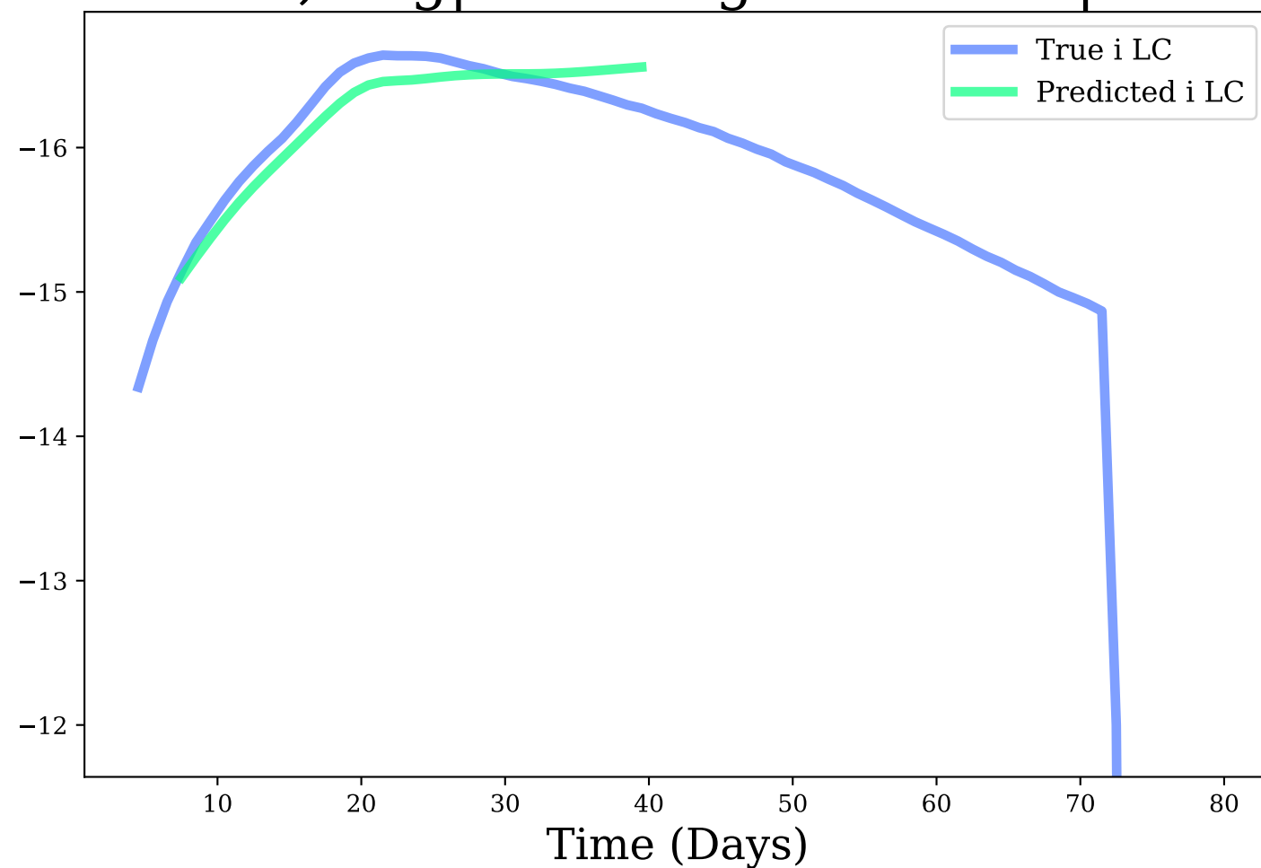
i-band, Avg|Max Mag Diff: 0.14 | 0.29
