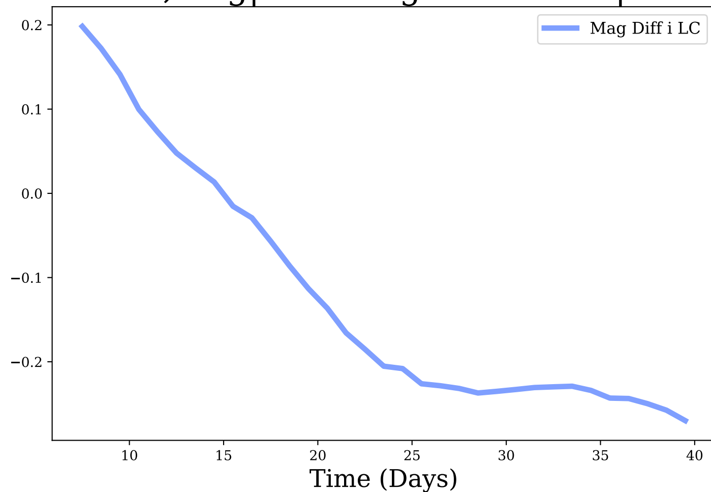
i-band, Avg|Max Mag Diff: -0.12 | 0.27
