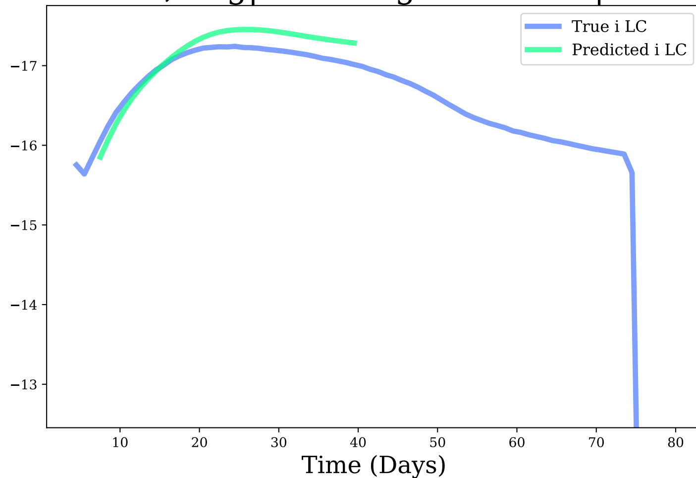
i-band, Avg|Max Mag Diff: 0.17 | 0.27
