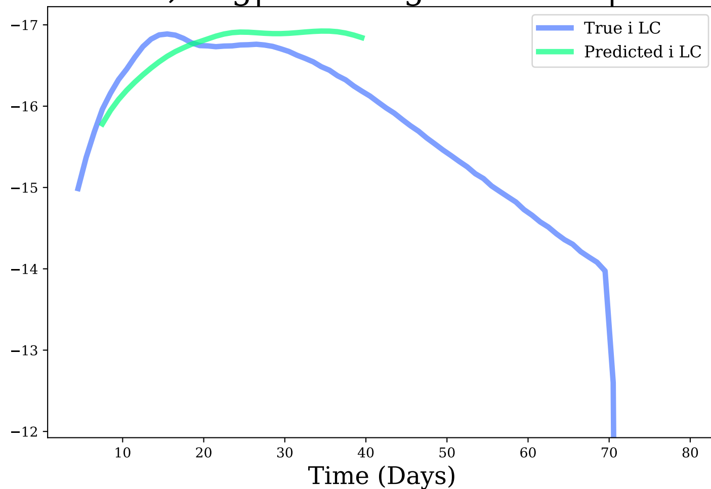
i-band, Avg|Max Mag Diff: 0.27 | 0.66
