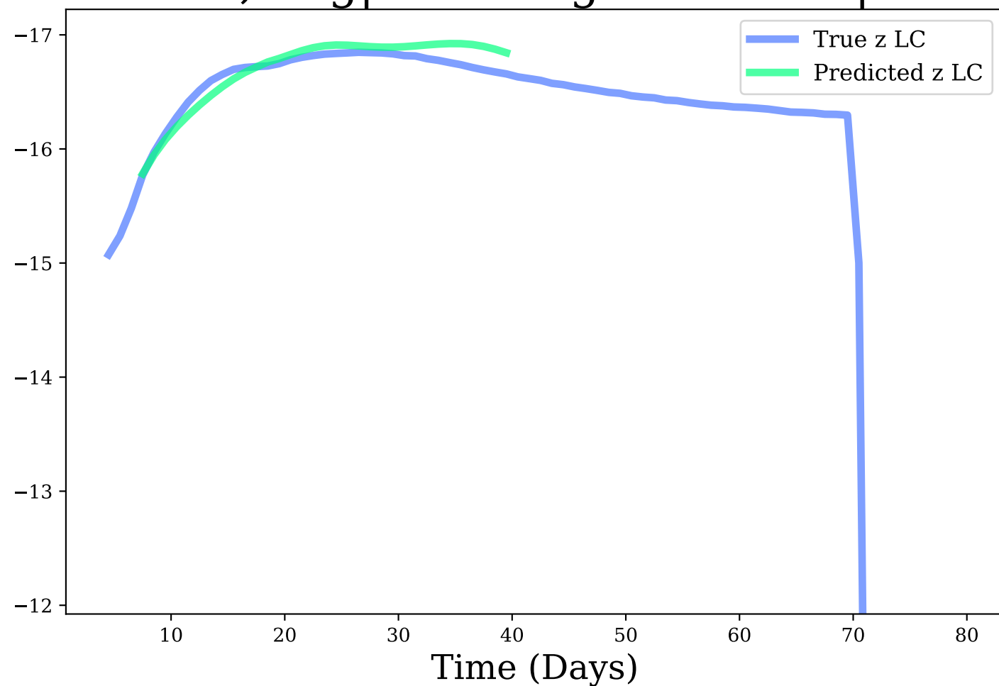
z-band, Avg|Max Mag Diff: 0.09 | 0.21
