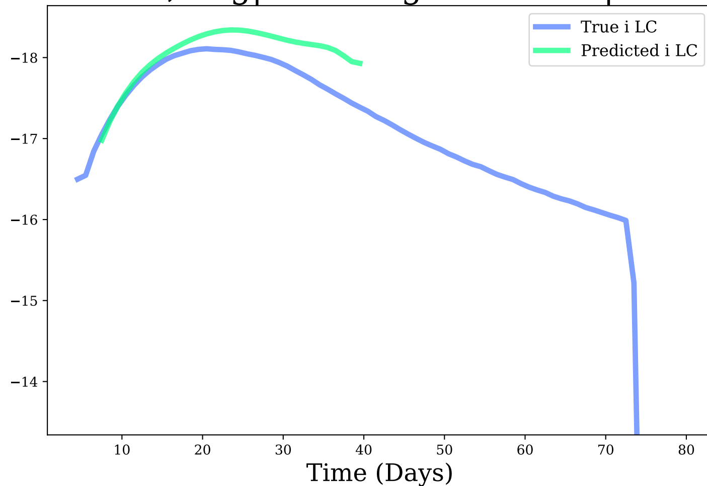
i-band, Avg|Max Mag Diff: 0.25 | 0.54
