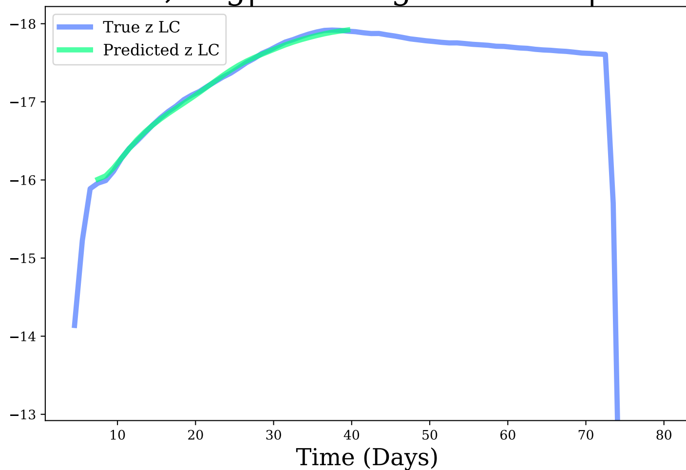
z-band, Avg|Max Mag Diff: 0.03 | 0.06
