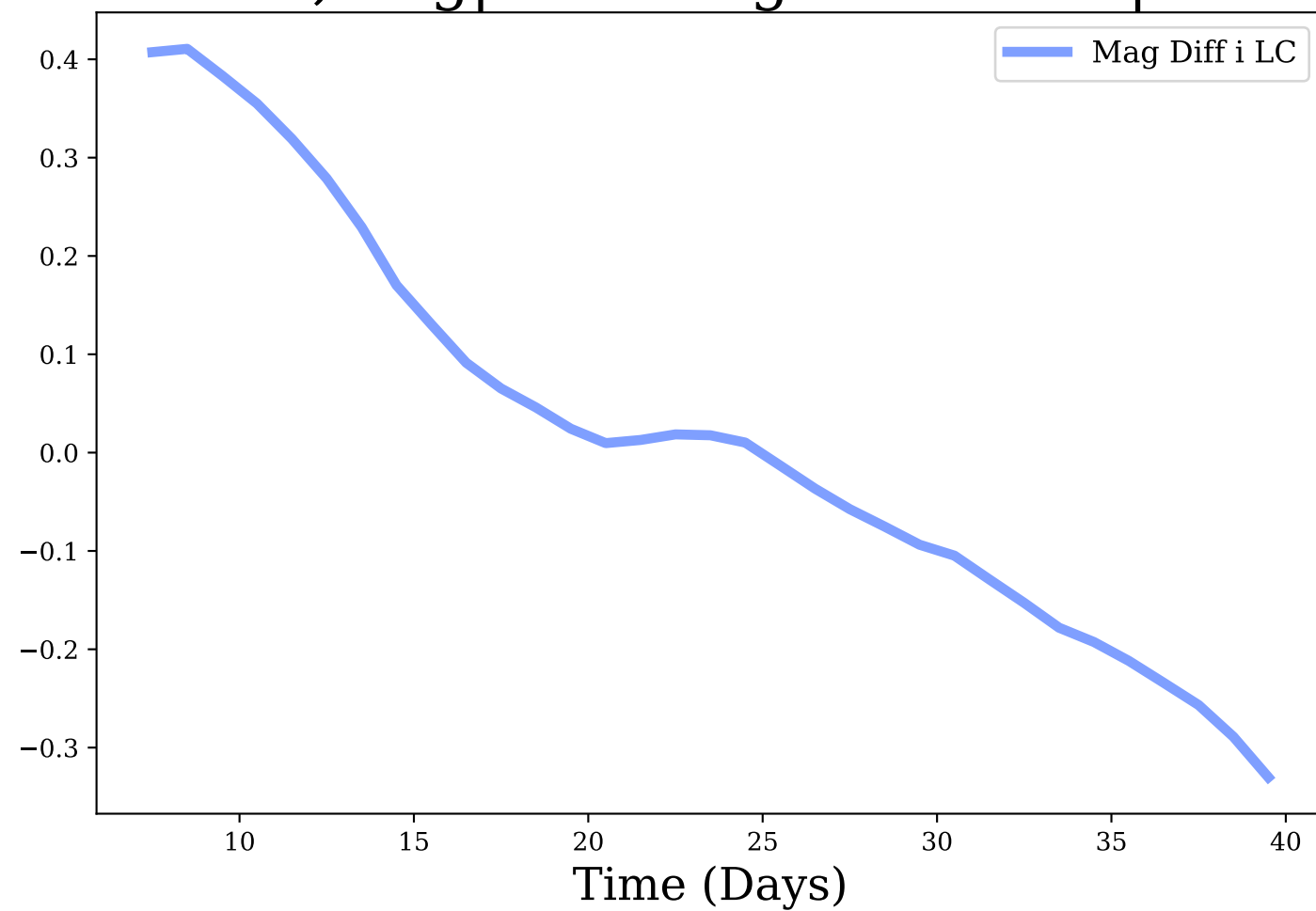
i-band, Avg|Max Mag Diff: 0.02 | 0.41
