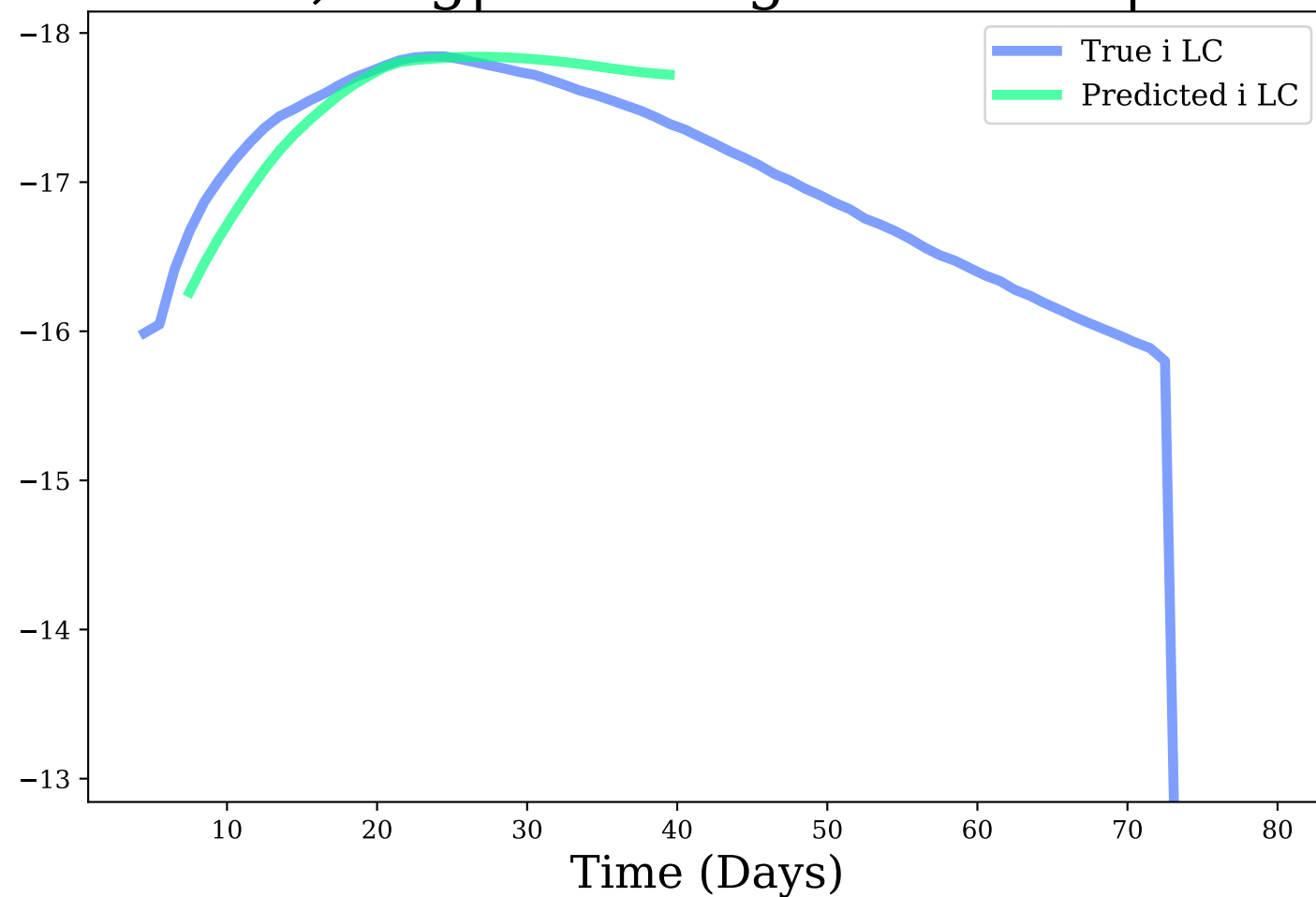
i-band, Avg|Max Mag Diff: 0.16 | 0.41
