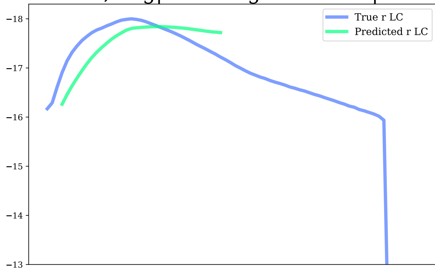
z-band, Avg|Max Mag Diff: 0.04 | 0.06
