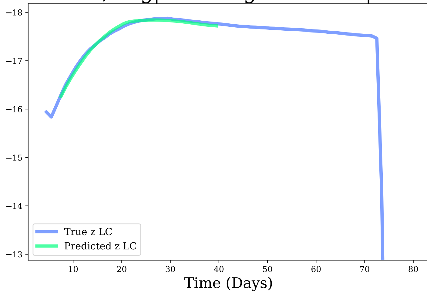
z-band, Avg|Max Mag Diff: 0.04 | 0.06
