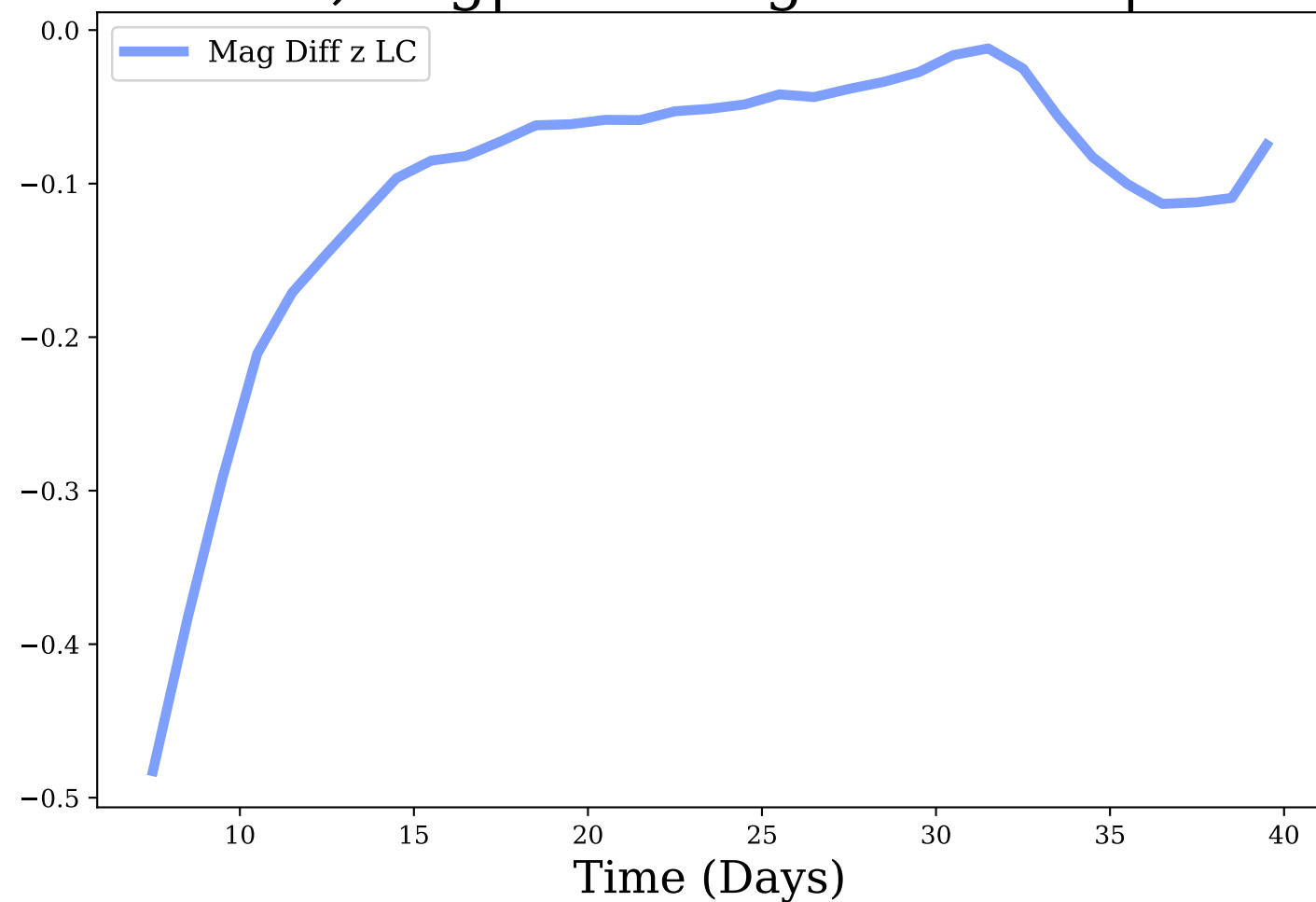
z-band, Avg|Max Mag Diff: -0.1 | 0.48
