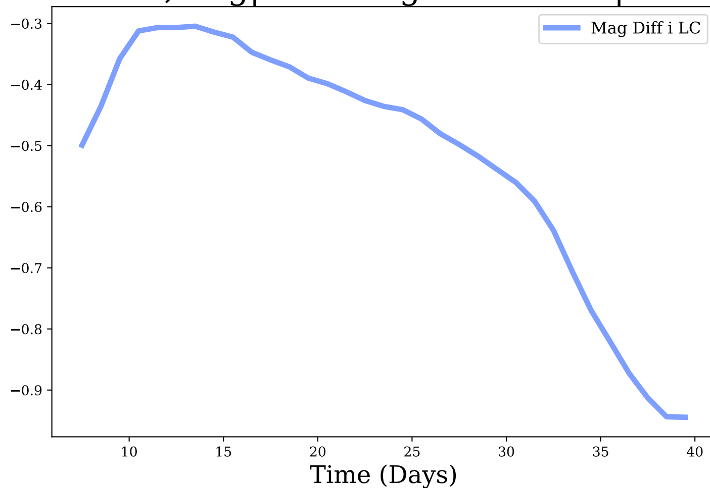
i-band, Avg|Max Mag Diff: -0.51 | 0.94
