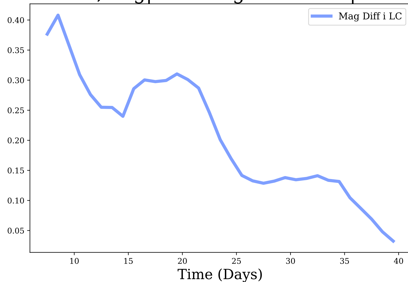
i-band, Avg|Max Mag Diff: 0.21 | 0.41
