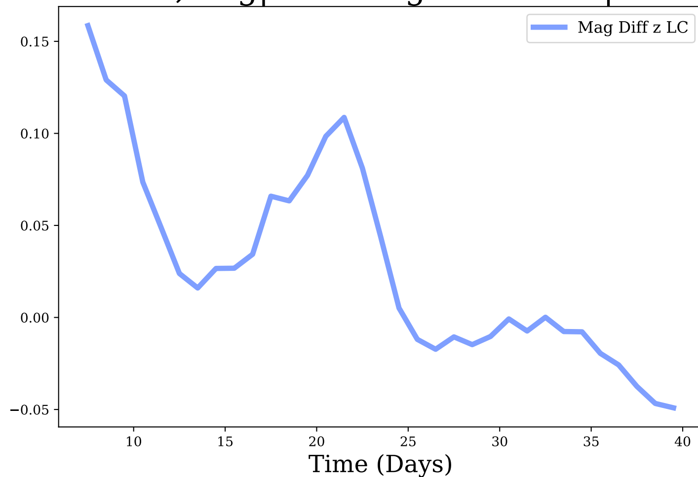
z-band, Avg|Max Mag Diff: 0.03 | 0.16
