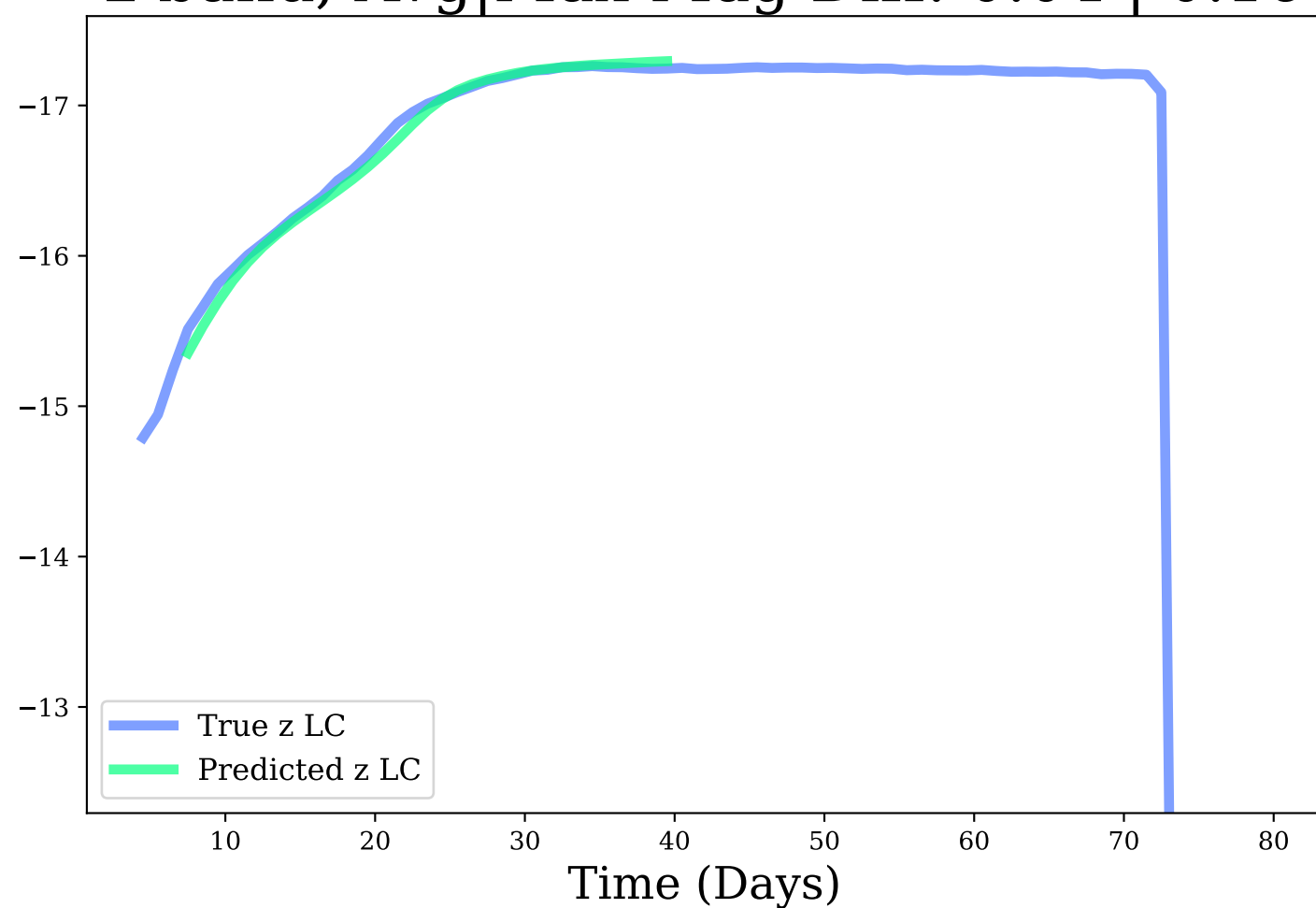
z-band, Avg|Max Mag Diff: 0.04 | 0.16
