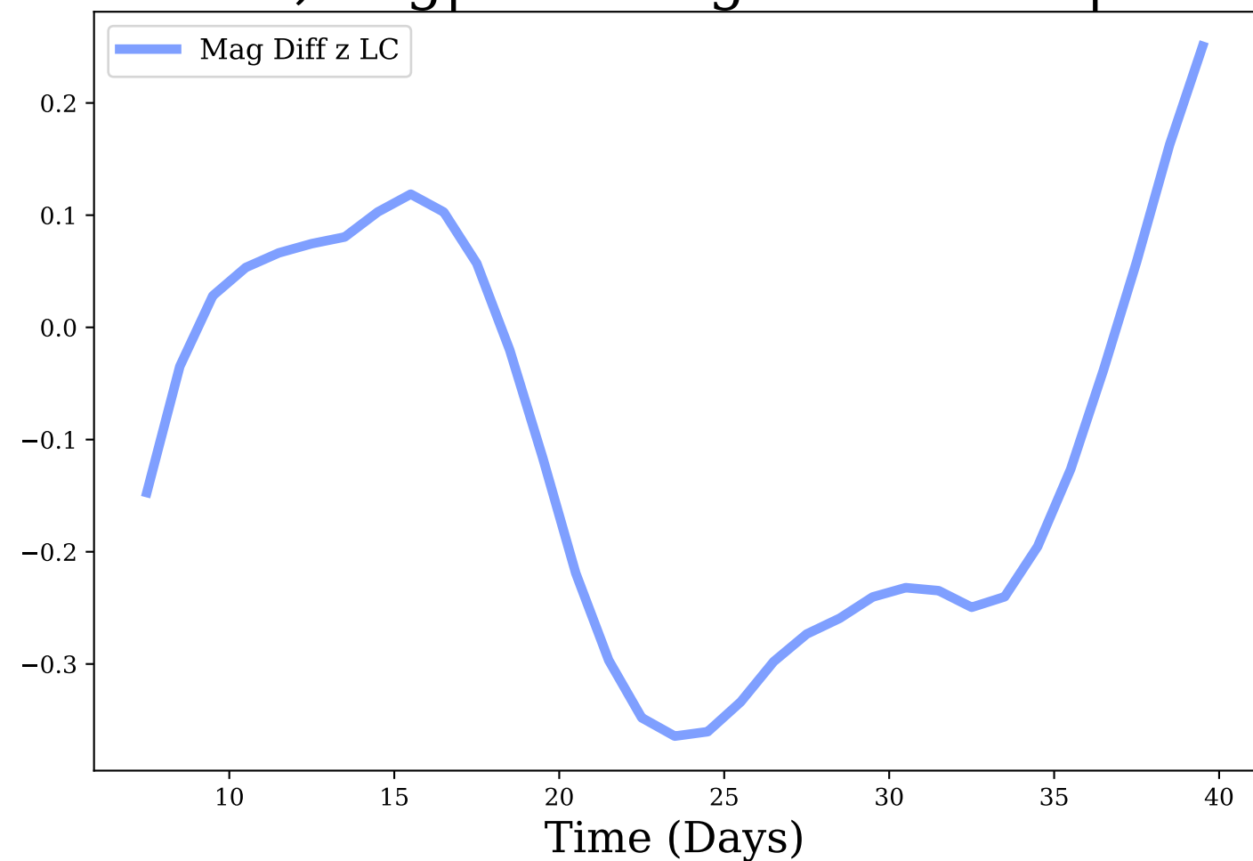
z-band, Avg|Max Mag Diff: -0.11 | 0.36
