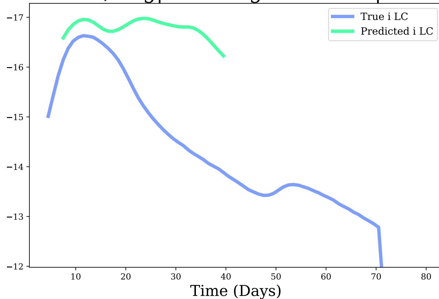
i-band, Avg|Max Mag Diff: 1.45 | 2.53
