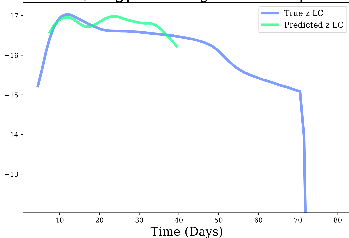
z-band, Avg|Max Mag Diff: 0.18 | 0.36
