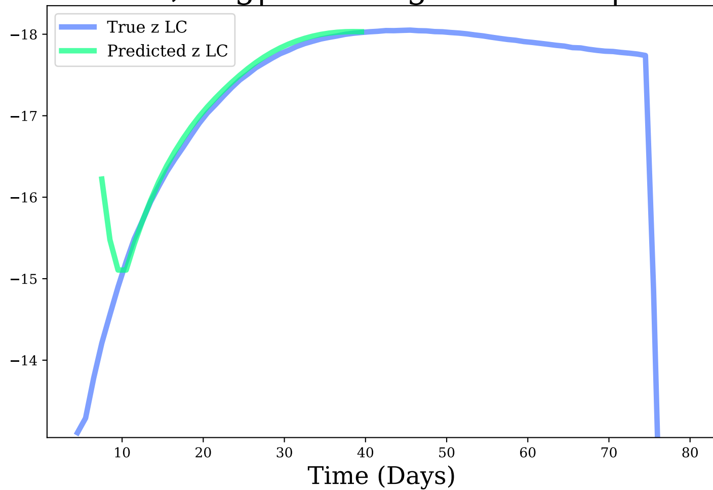
z-band, Avg|Max Mag Diff: 0.15 | 2.01
