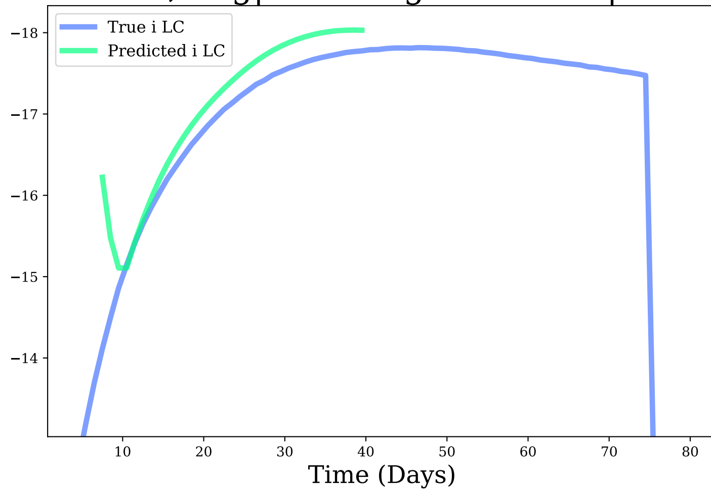
i-band, Avg|Max Mag Diff: 0.32 | 2.11
