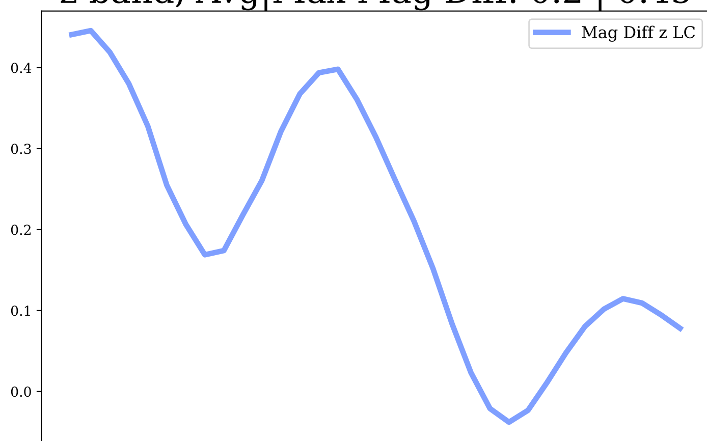
z-band, Avg|Max Mag Diff: 0.2 | 0.45
