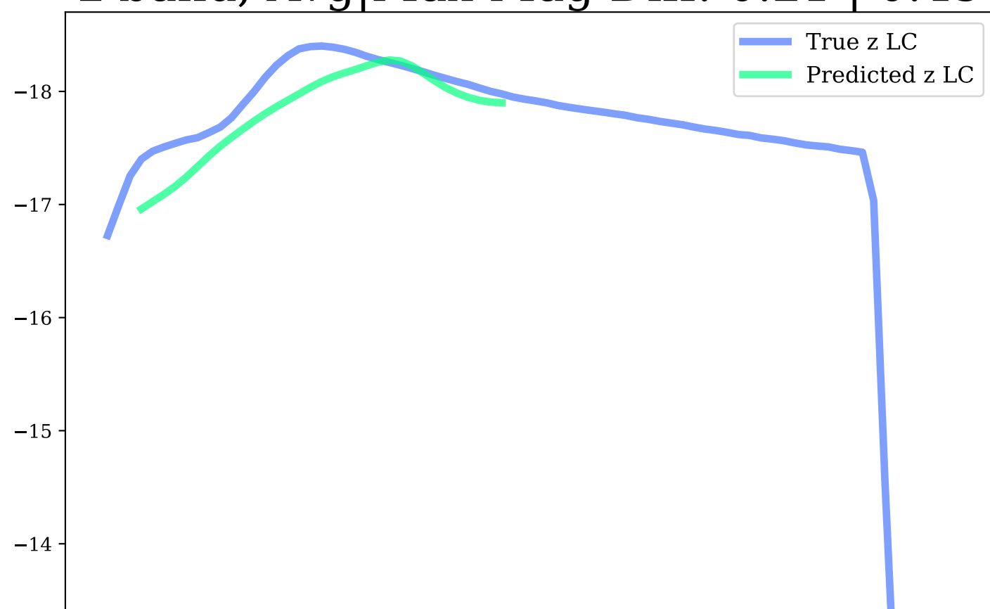
z-band, Avg|Max Mag Diff: 0.21 | 0.45
