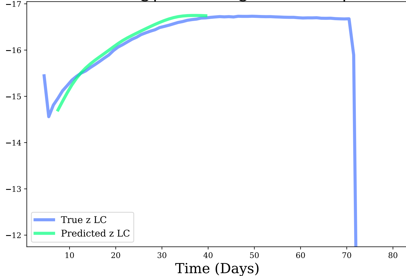
z-band, Avg|Max Mag Diff: 0.1 | 0.25
