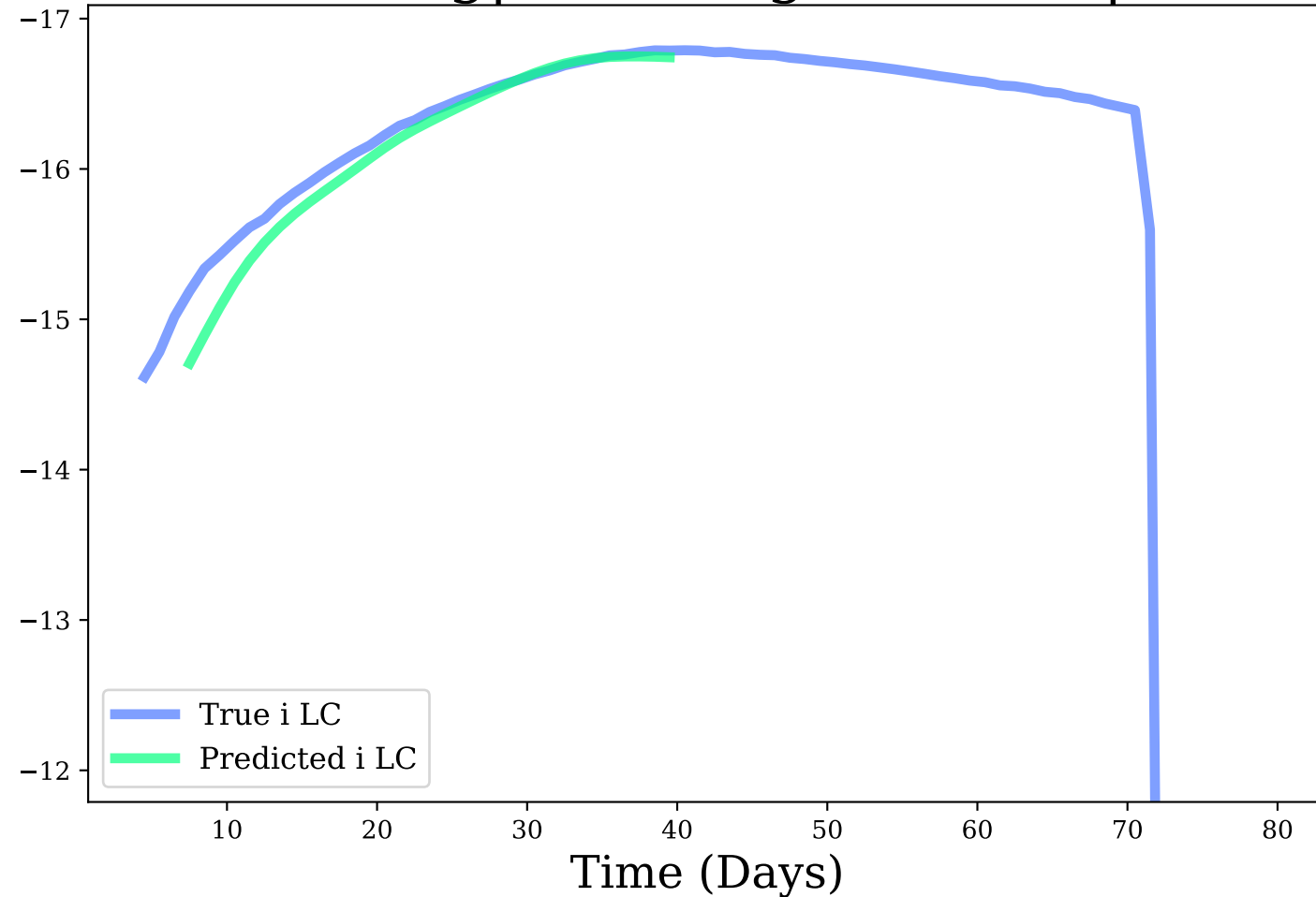
i-band, Avg|Max Mag Diff: 0.1 | 0.48
