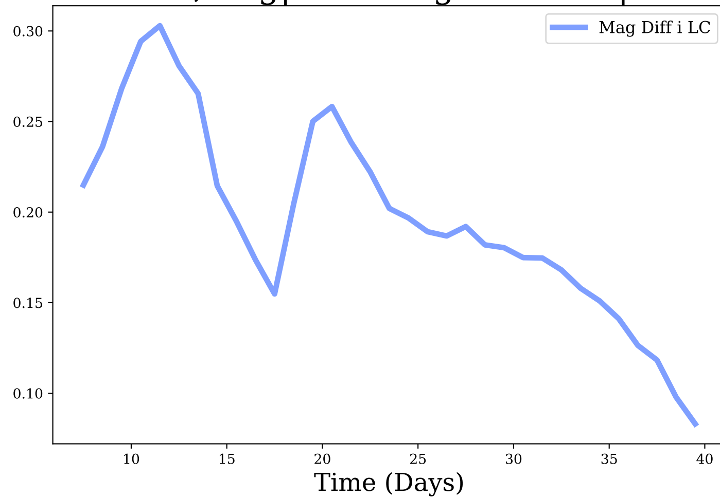
i-band, Avg|Max Mag Diff: 0.2 | 0.3
