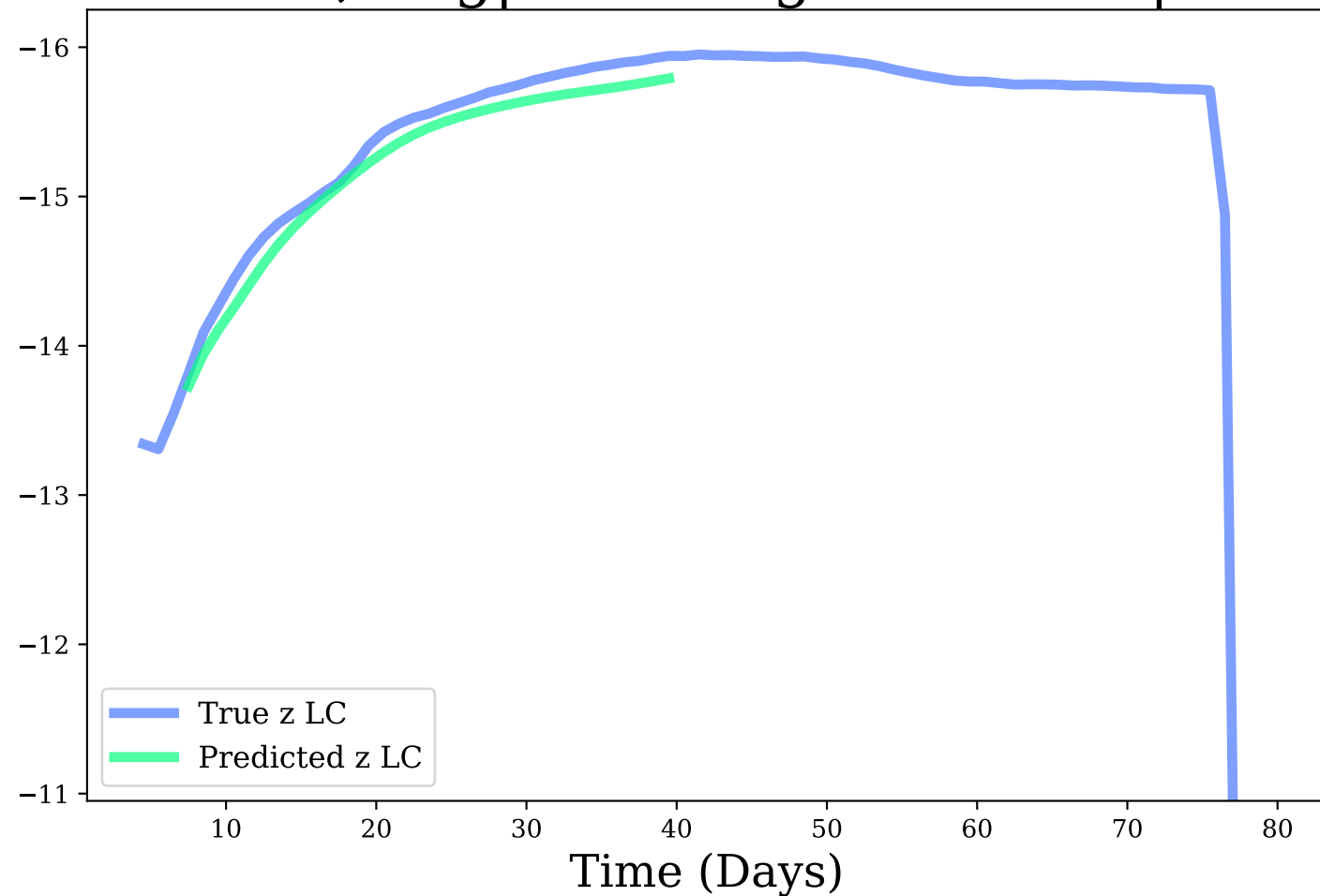
z-band, Avg|Max Mag Diff: 0.12 | 0.2
