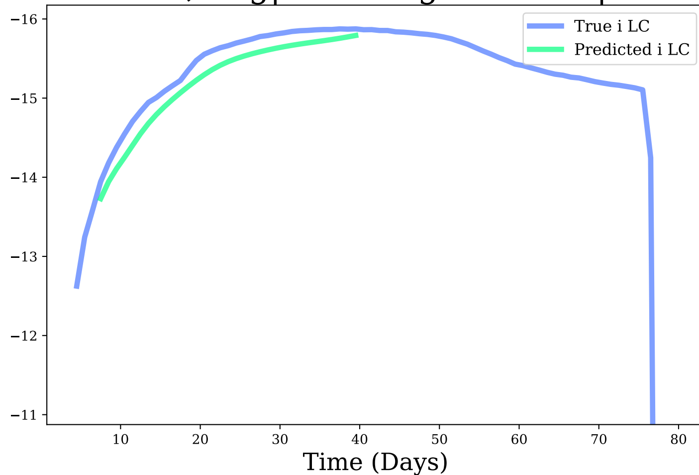
i-band, Avg|Max Mag Diff: 0.2 | 0.3
