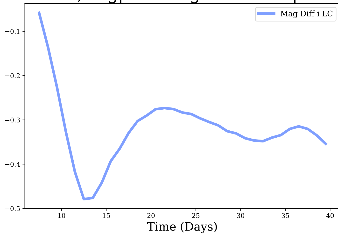
i-band, Avg|Max Mag Diff: -0.32 | 0.48
