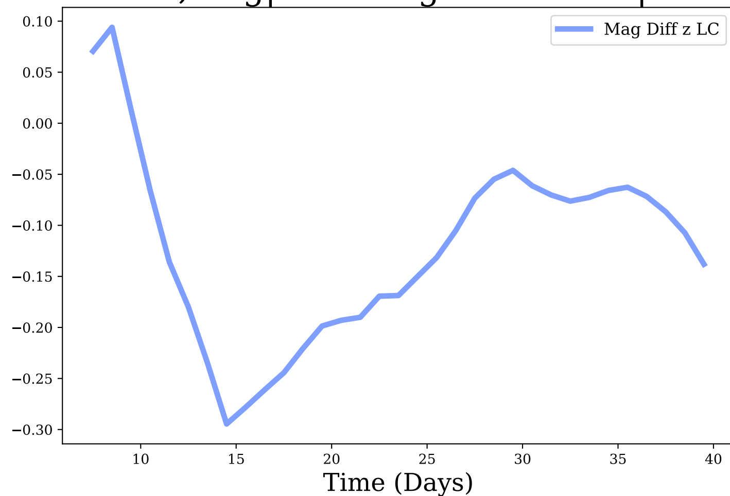
z-band, Avg|Max Mag Diff: -0.12 | 0.29
