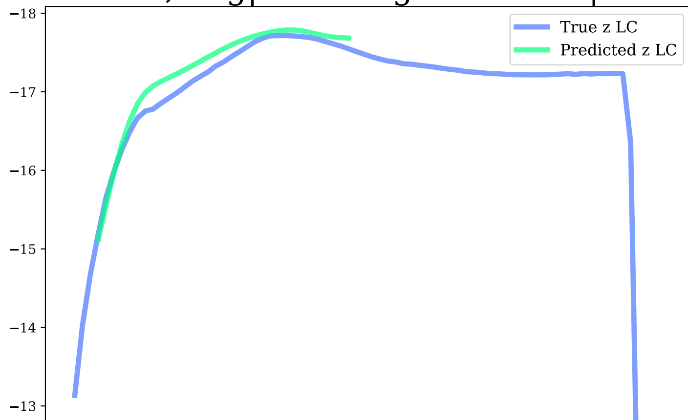
z-band, Avg|Max Mag Diff: 0.13 | 0.29
