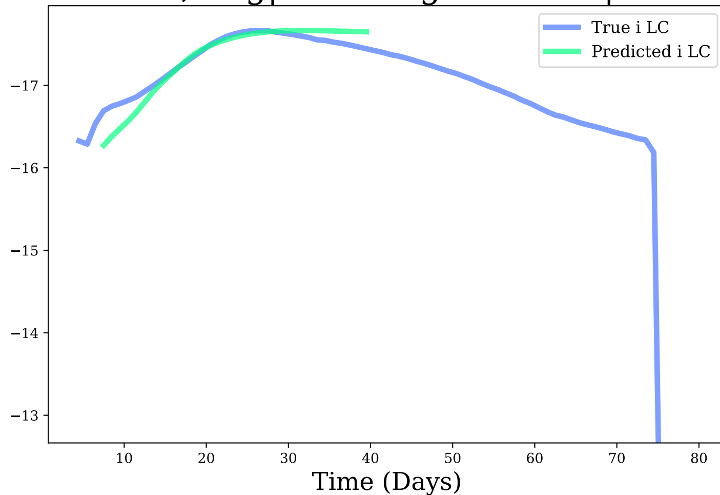
i-band, Avg|Max Mag Diff: 0.1 | 0.42
