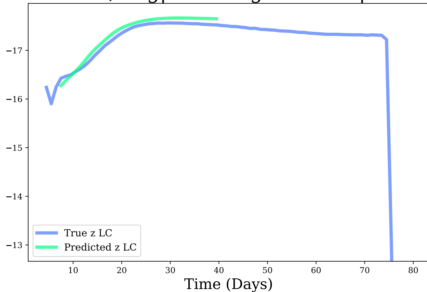
z-band, Avg|Max Mag Diff: 0.1 | 0.15
