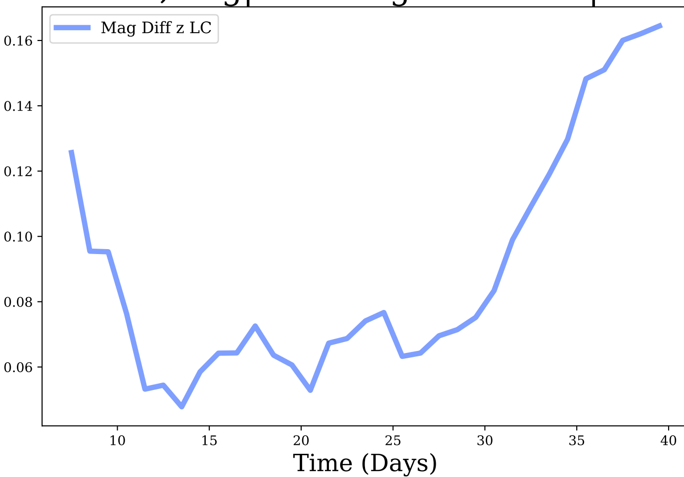
z-band, Avg|Max Mag Diff: 0.09 | 0.16
