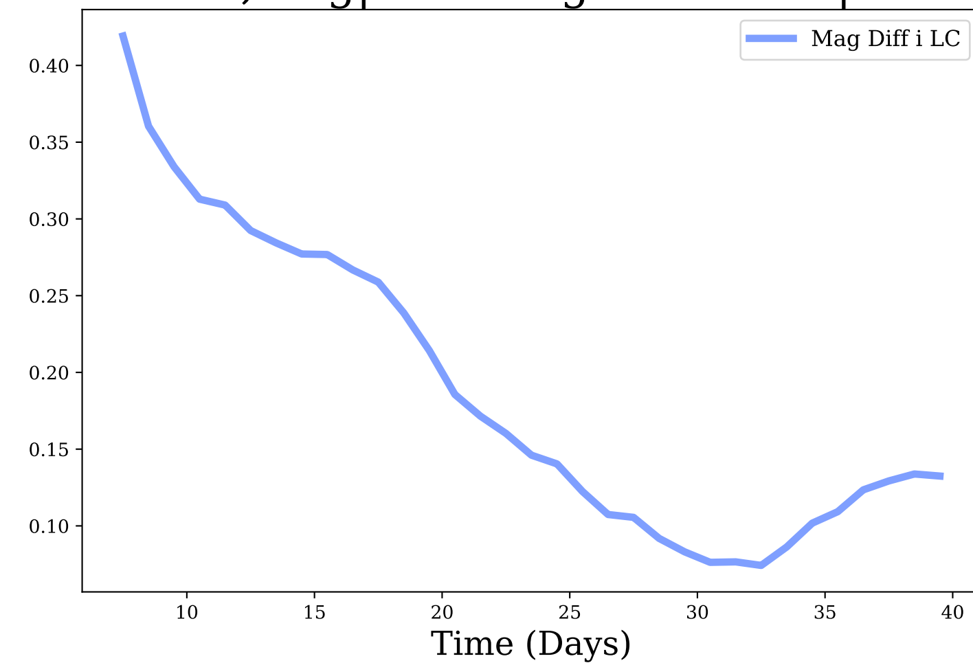
i-band, Avg|Max Mag Diff: 0.19 | 0.42
