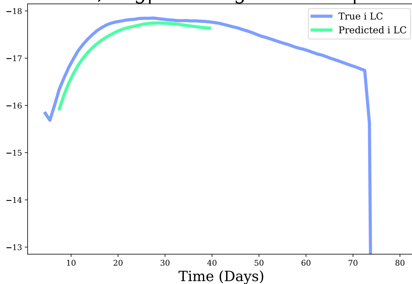
i-band, Avg|Max Mag Diff: 0.19 | 0.42
