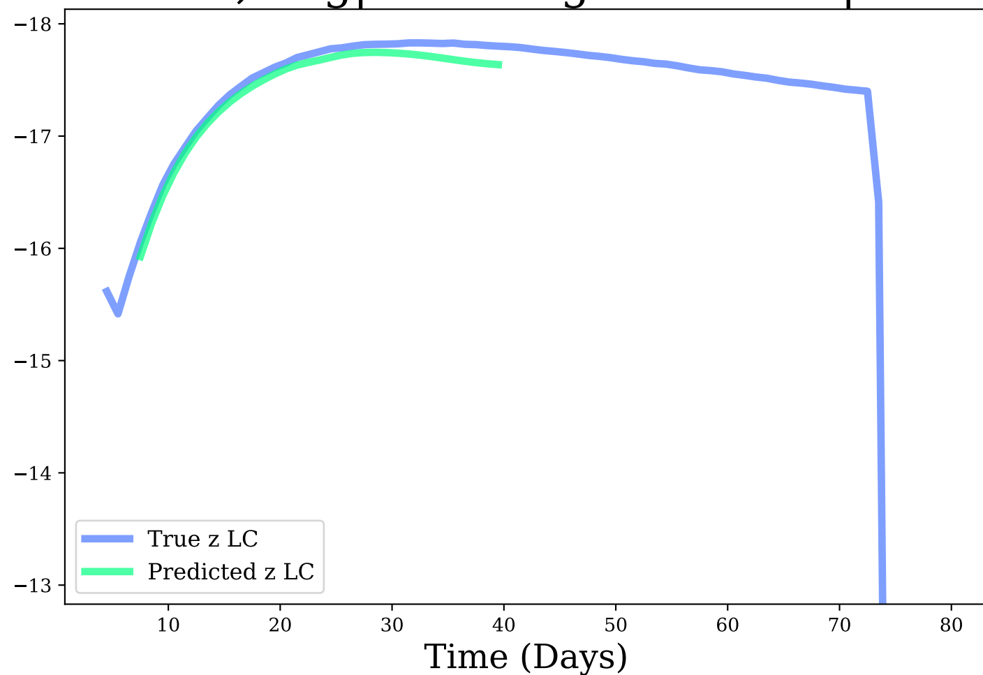
z-band, Avg|Max Mag Diff: 0.09 | 0.16
