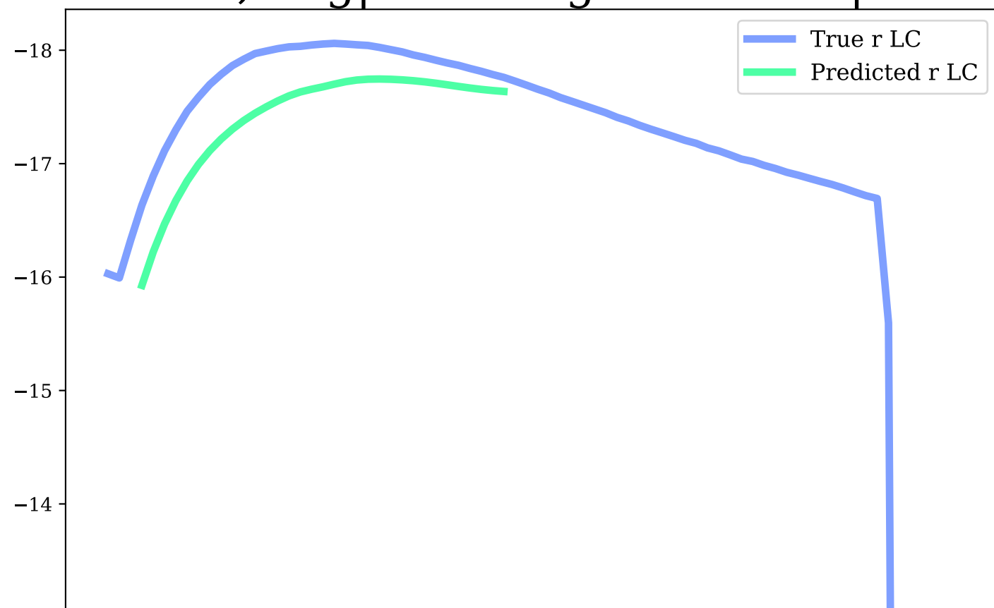
z-band, Avg|Max Mag Diff: 0.09 | 0.16
