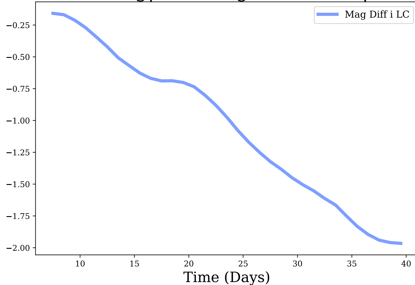
i-band, Avg|Max Mag Diff: -1.05 | 1.97
