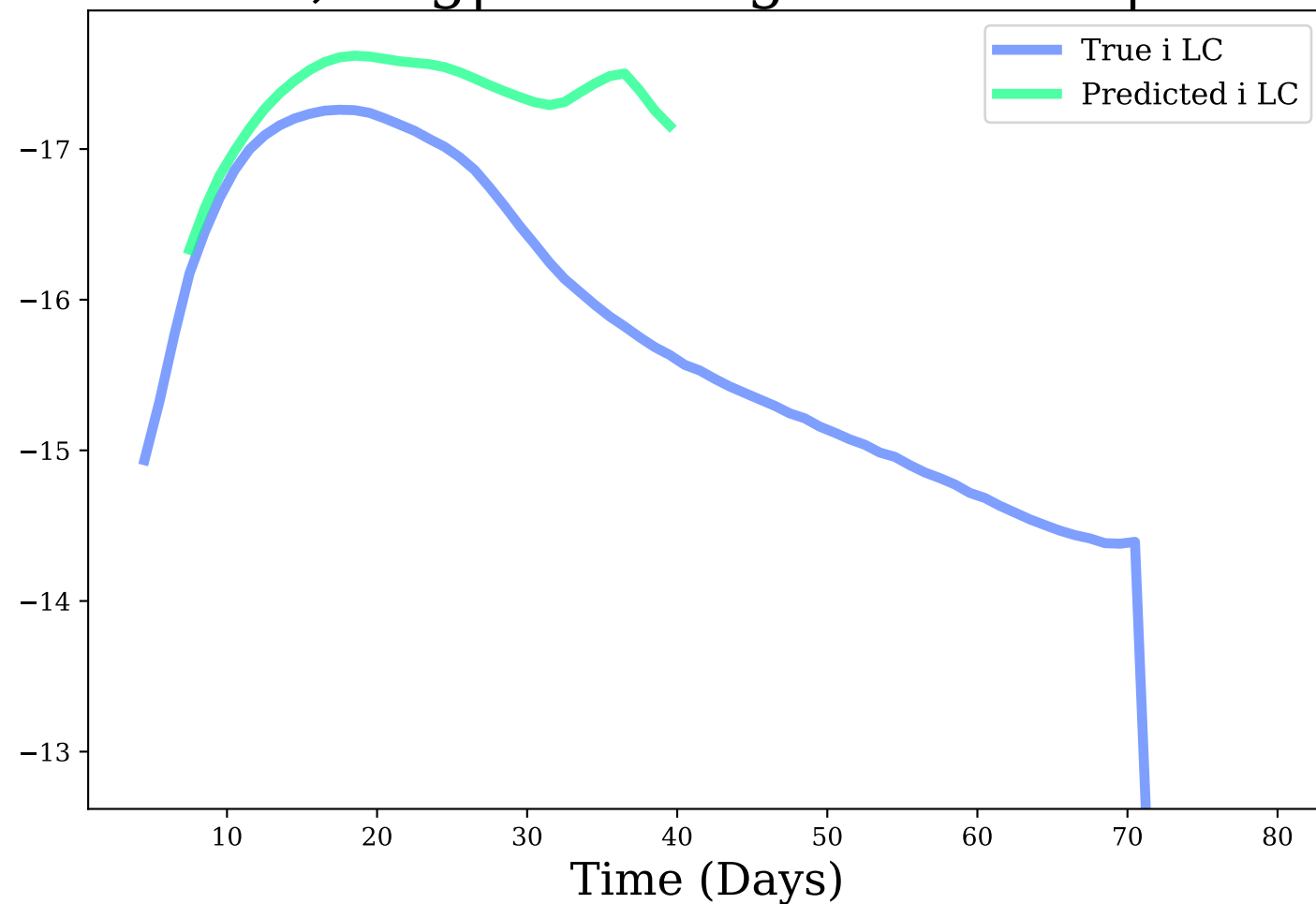
i-band, Avg|Max Mag Diff: 0.69 | 1.68
