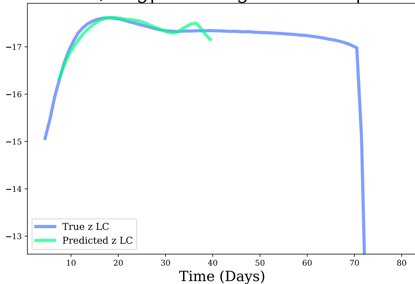
z-band, Avg|Max Mag Diff: 0.07 | 0.19
