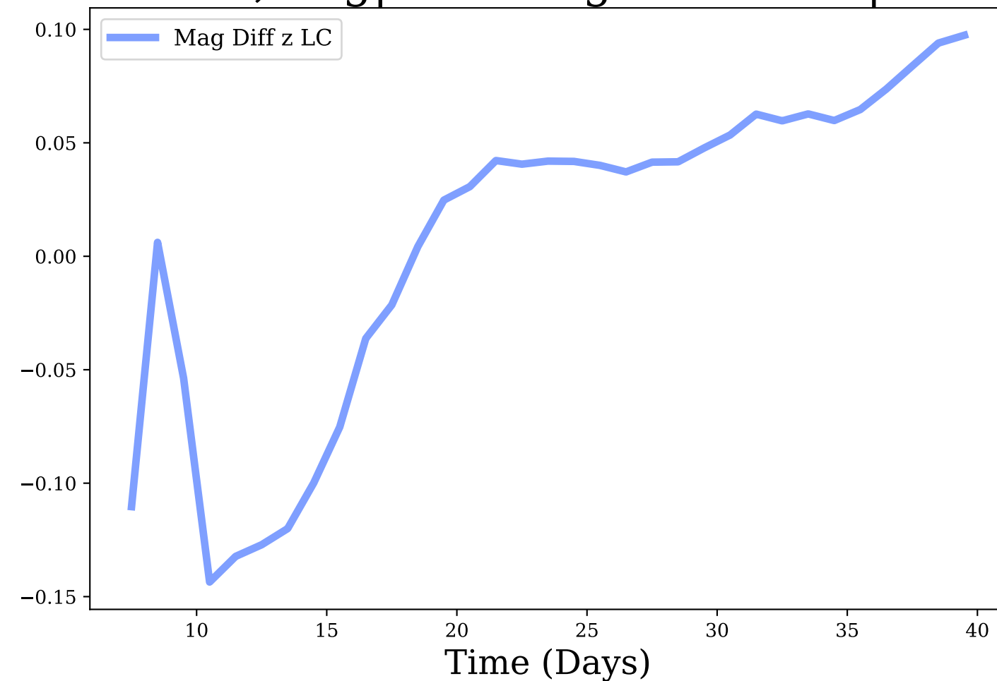
z-band, Avg|Max Mag Diff: 0.01 | 0.14
