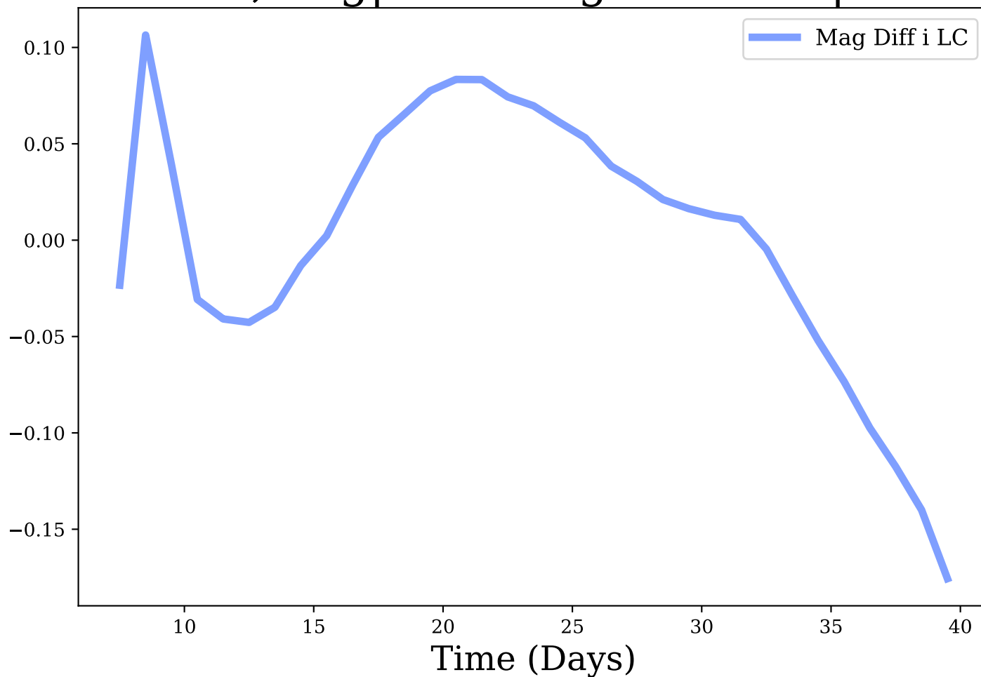
i-band, Avg|Max Mag Diff: 0.0 | 0.18
