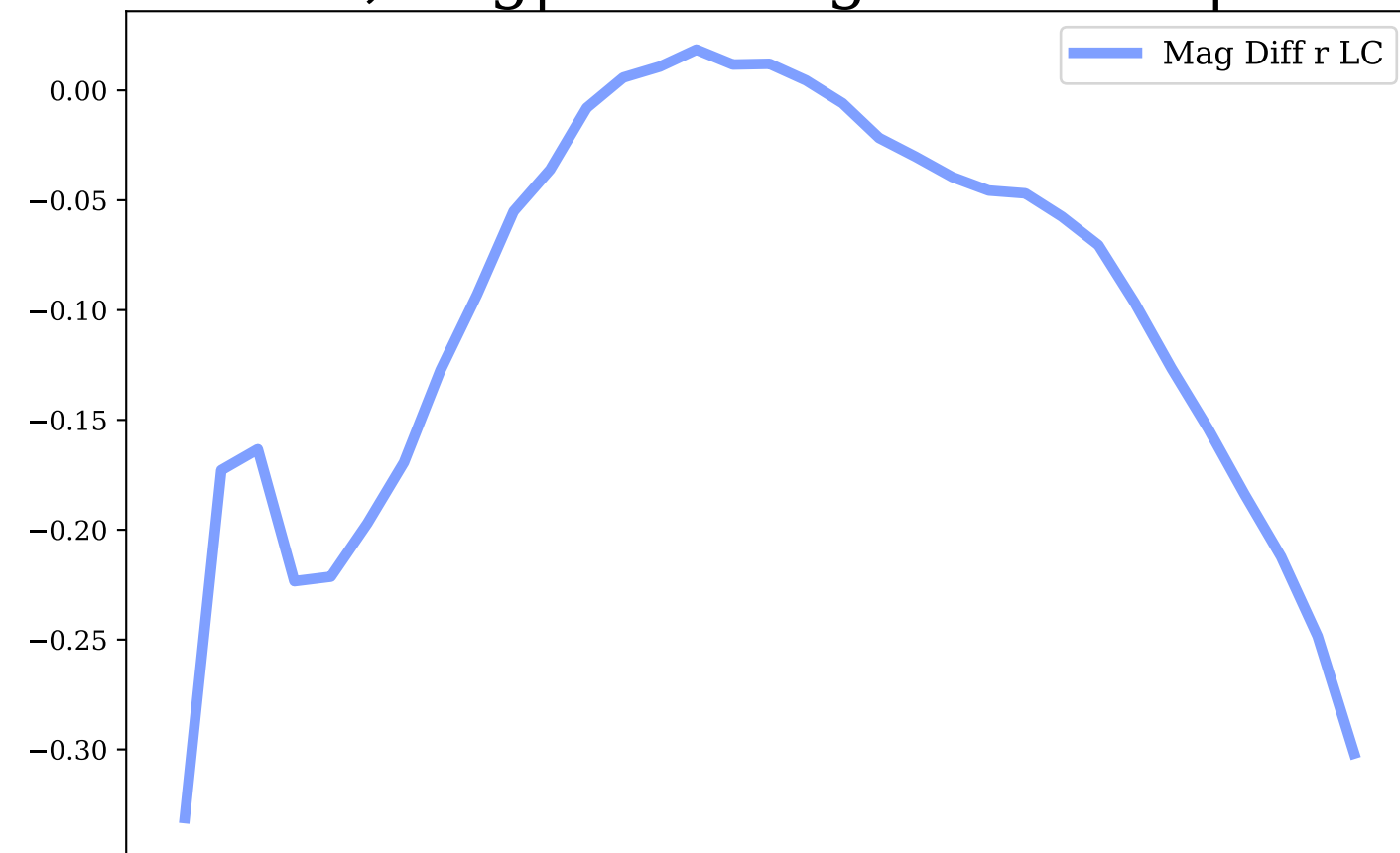
z-band, Avg|Max Mag Diff: 0.01 | 0.14
