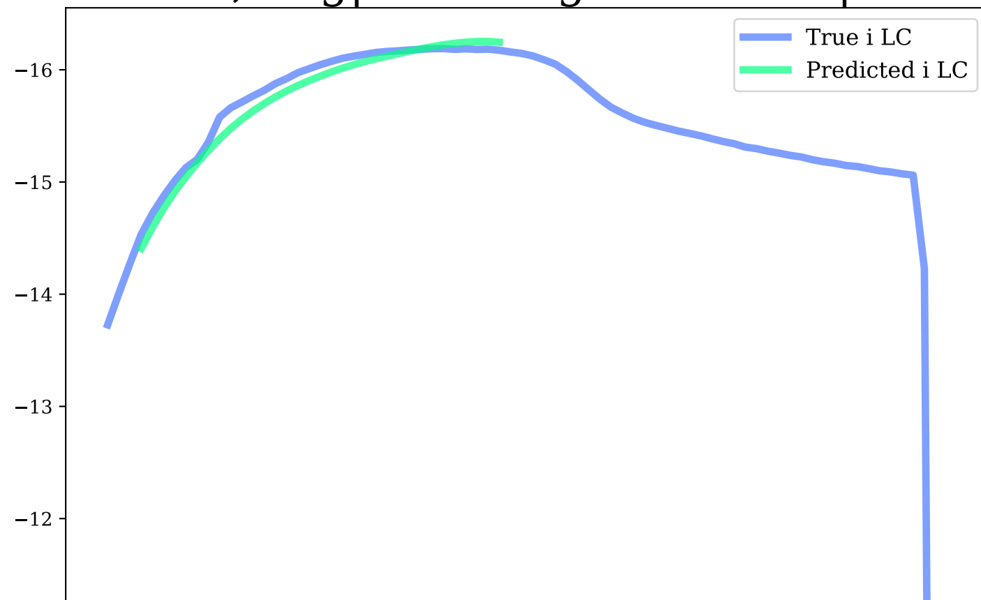
i-band, Avg|Max Mag Diff: 0.09 | 0.19
