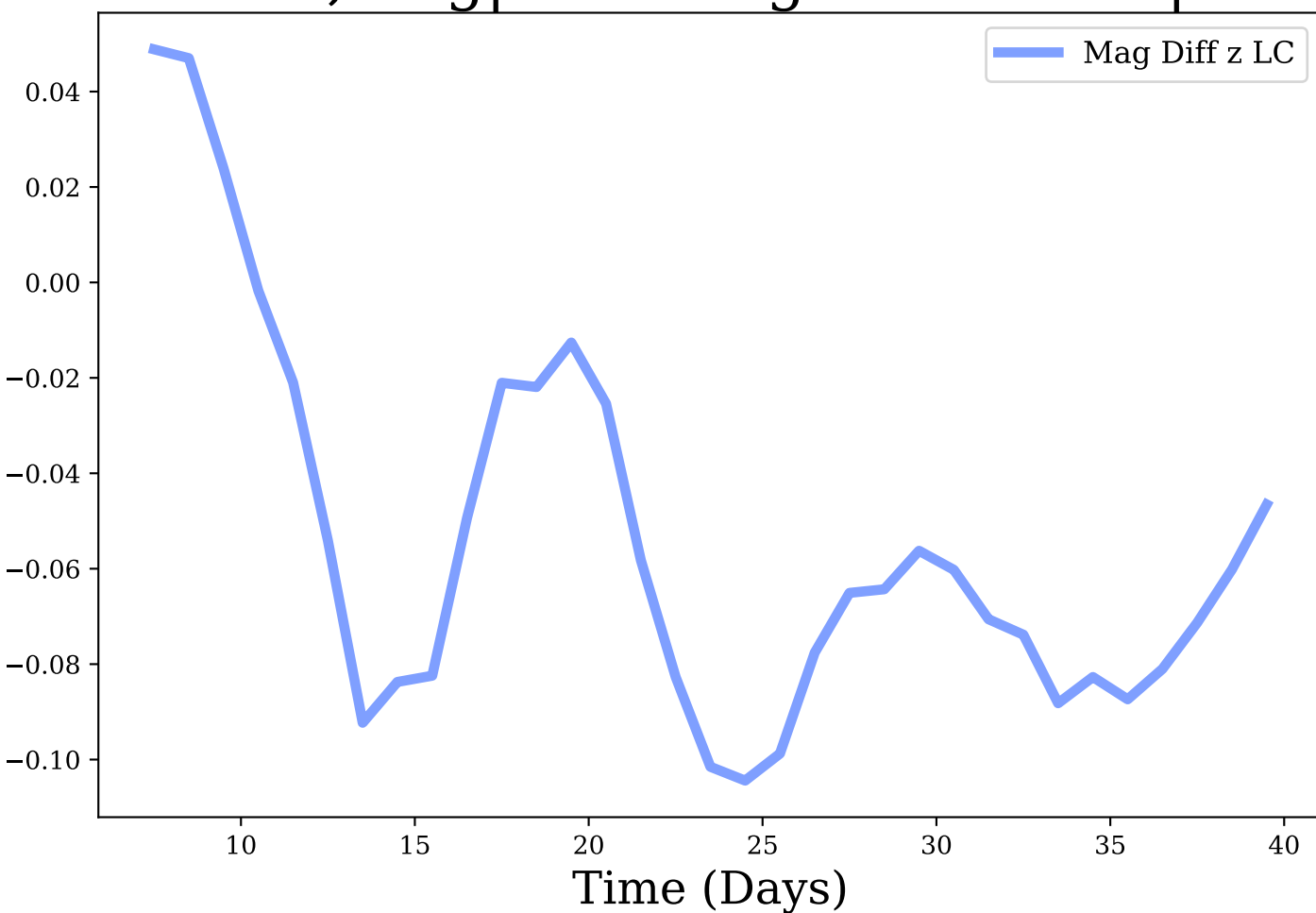
z-band, Avg|Max Mag Diff: -0.05 | 0.1
