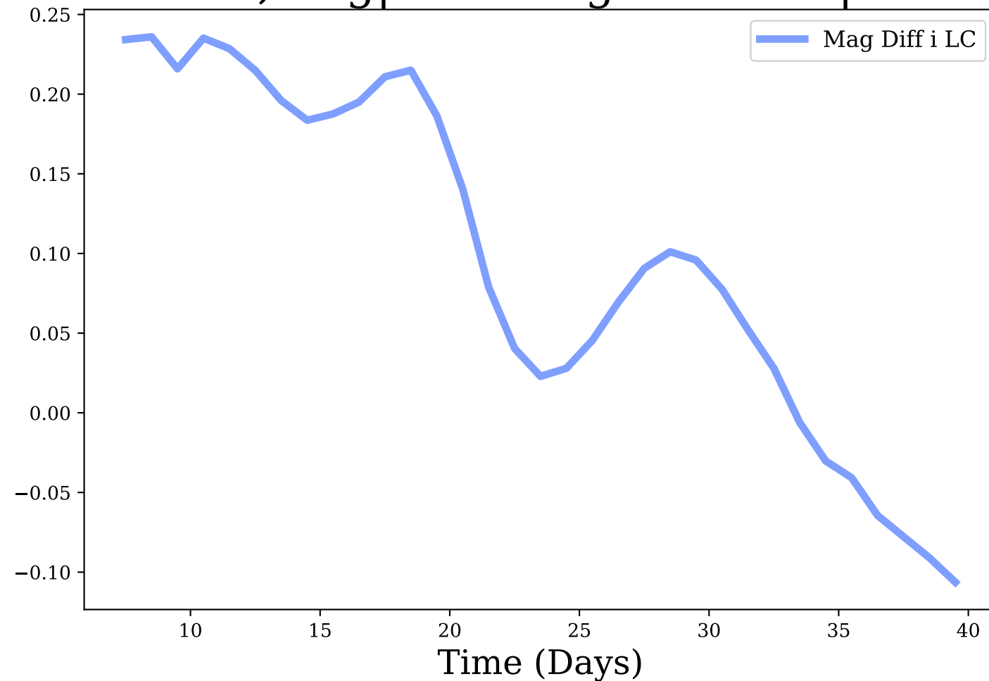
i-band, Avg|Max Mag Diff: 0.1 | 0.24
