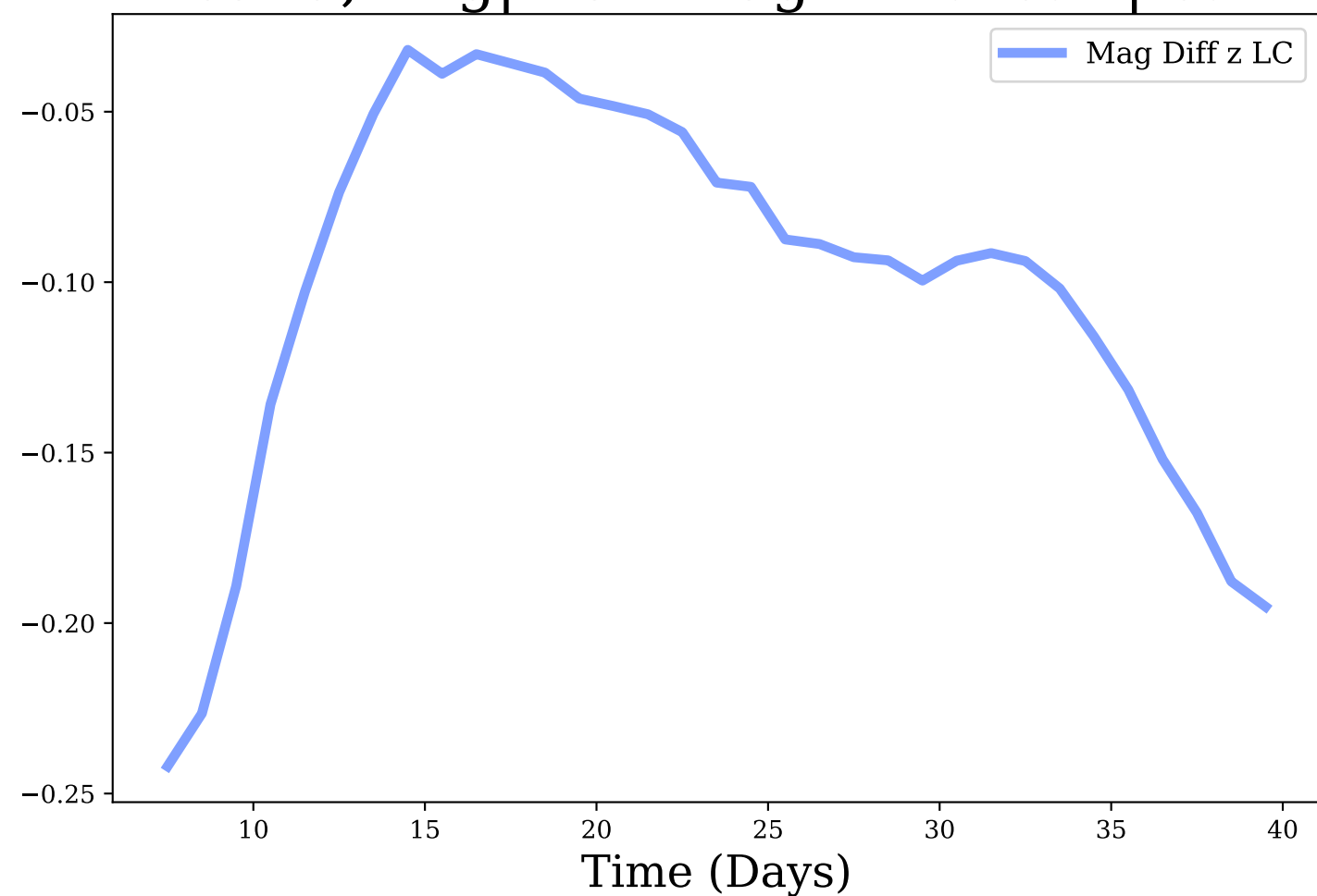
z-band, Avg|Max Mag Diff: -0.1 | 0.24
