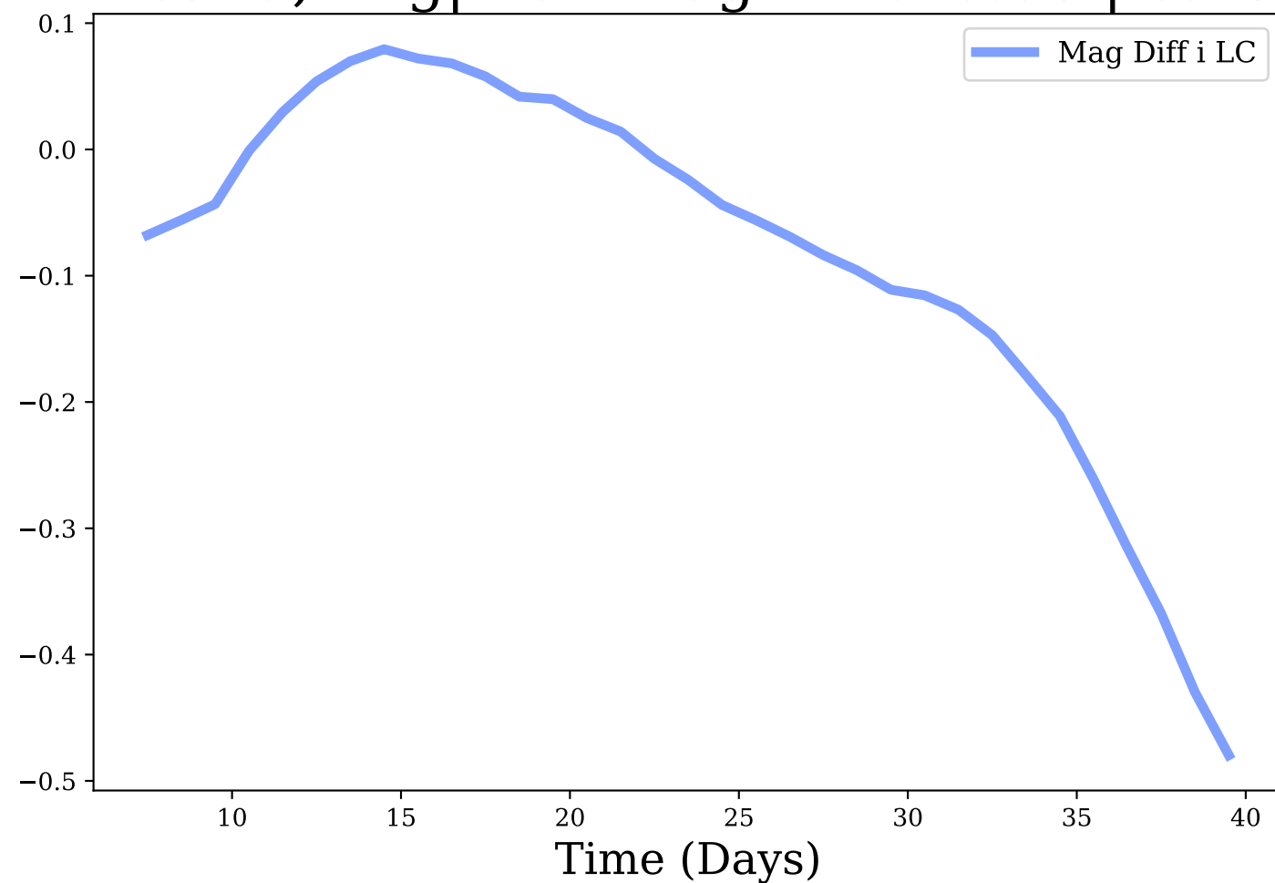
i-band, Avg|Max Mag Diff: -0.08 | 0.48
