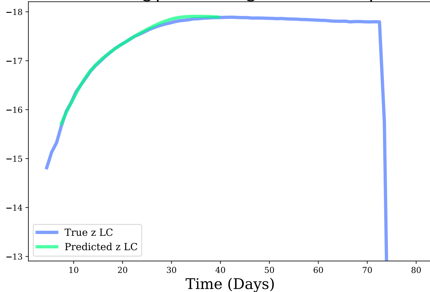
z-band, Avg|Max Mag Diff: 0.03 | 0.07
