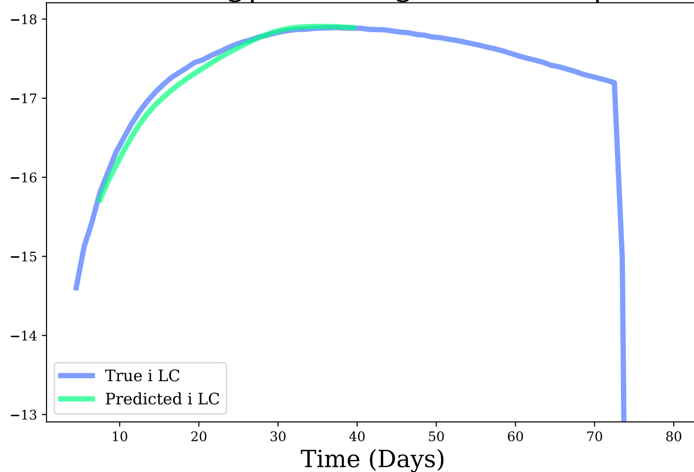
i-band, Avg|Max Mag Diff: 0.08 | 0.17
