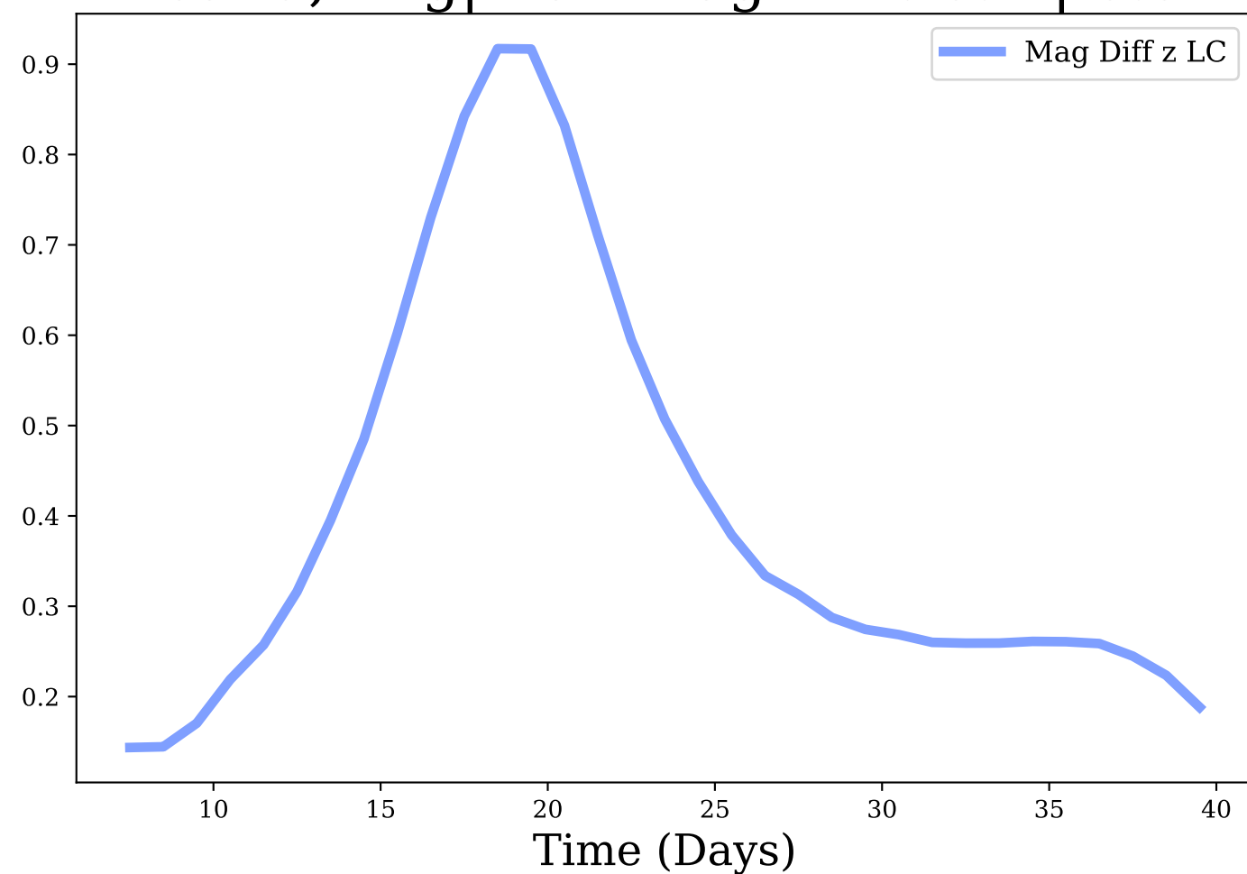
z-band, Avg|Max Mag Diff: 0.4 | 0.92
