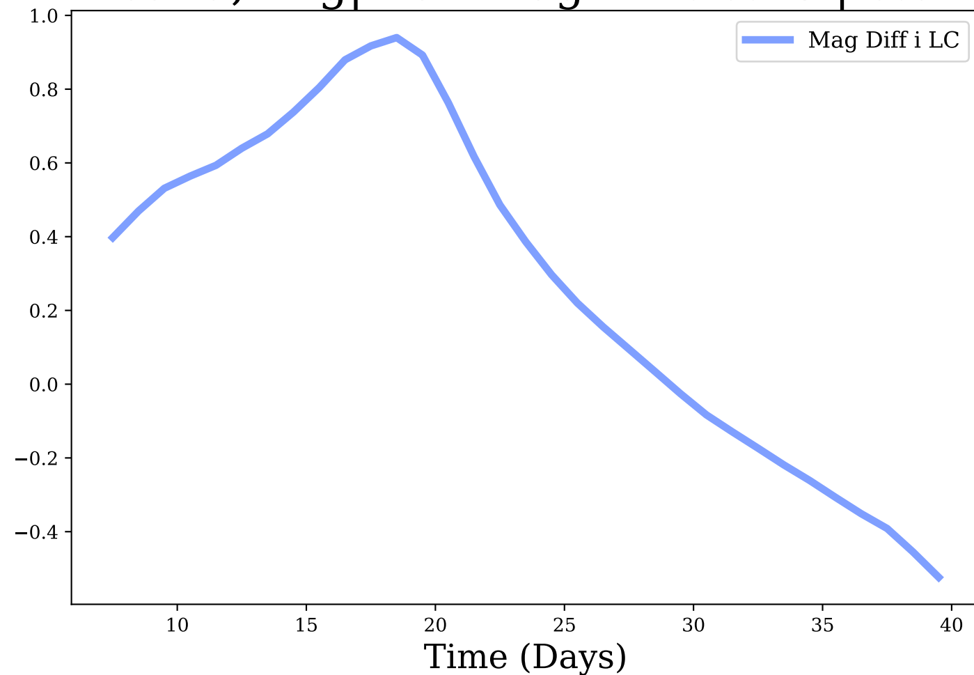
i-band, Avg|Max Mag Diff: 0.28 | 0.94
