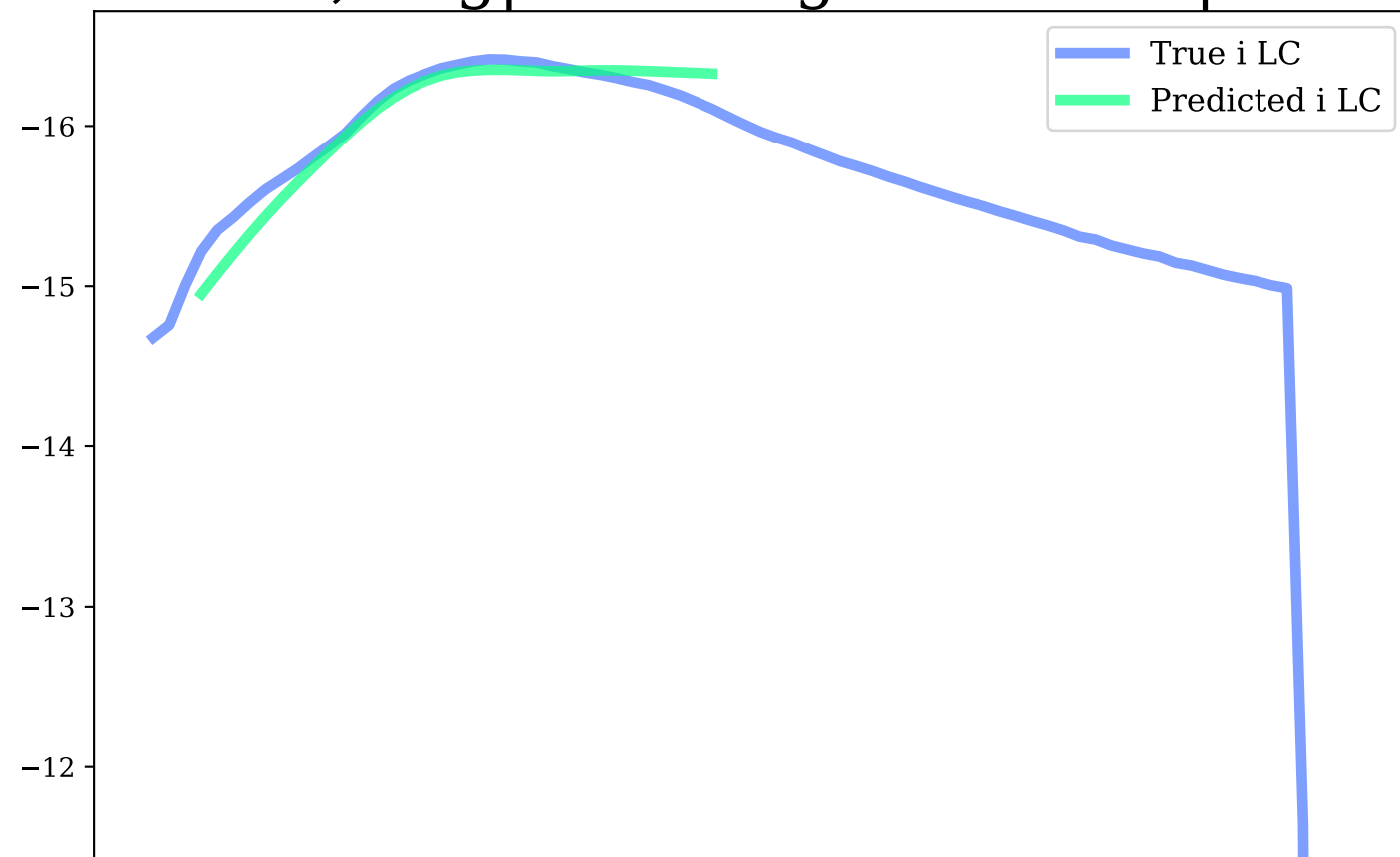
i-band, Avg|Max Mag Diff: 0.09 | 0.27
