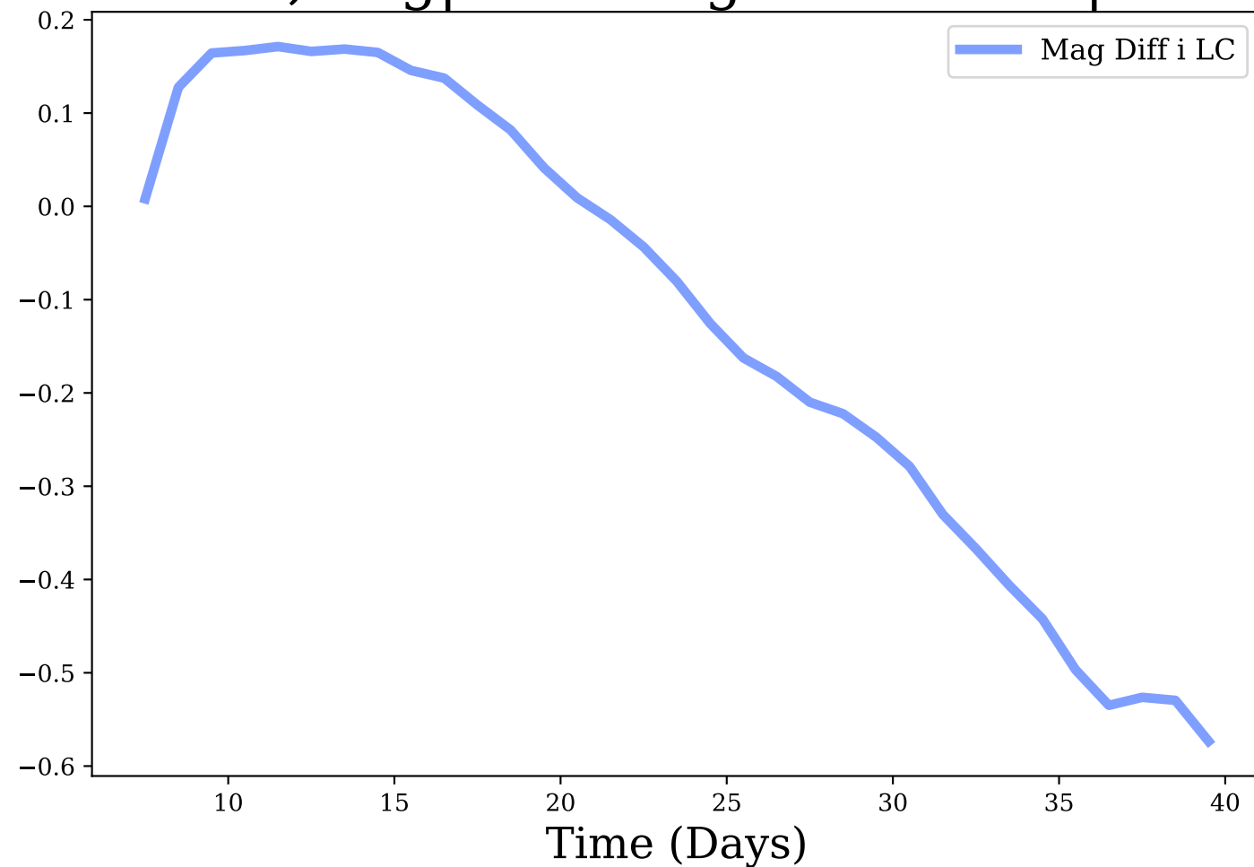
i-band, Avg|Max Mag Diff: -0.12 | 0.57
