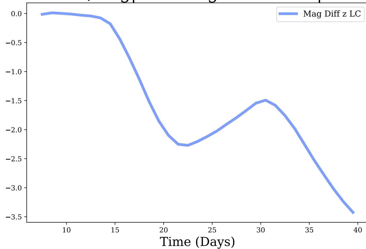
z-band, Avg|Max Mag Diff: -1.51 | 3.42
