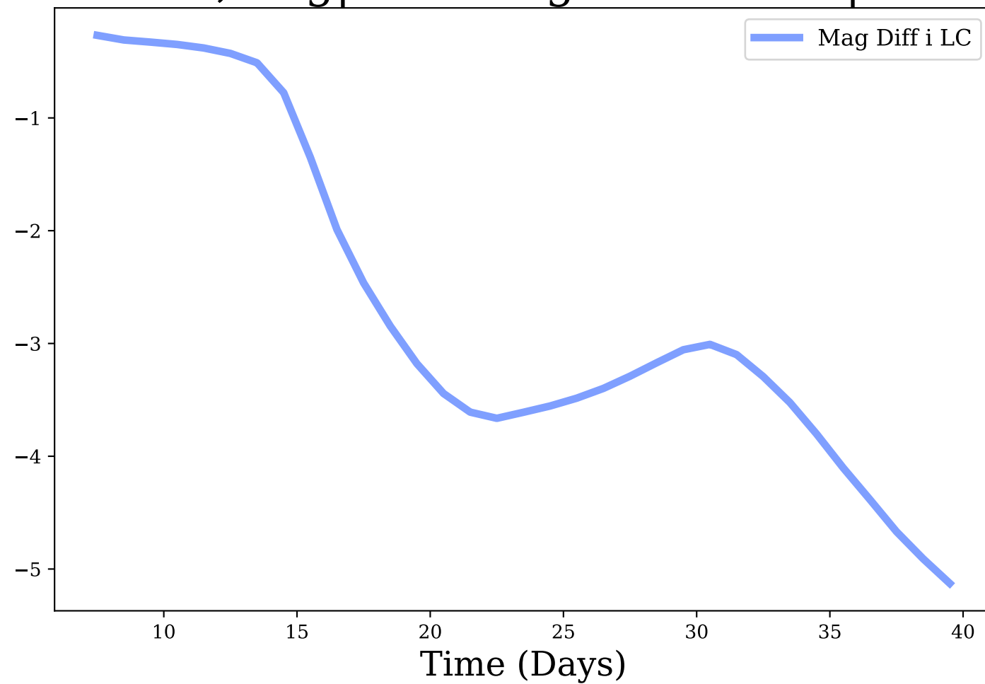
i-band, Avg|Max Mag Diff: -2.71 | 5.13
