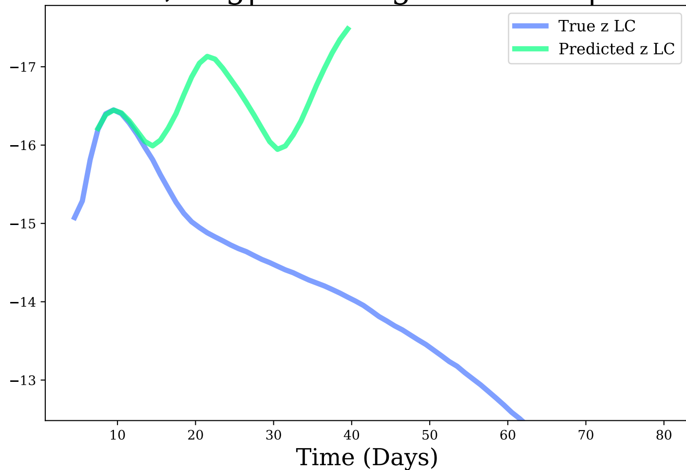
z-band, Avg|Max Mag Diff: 1.51 | 3.42
