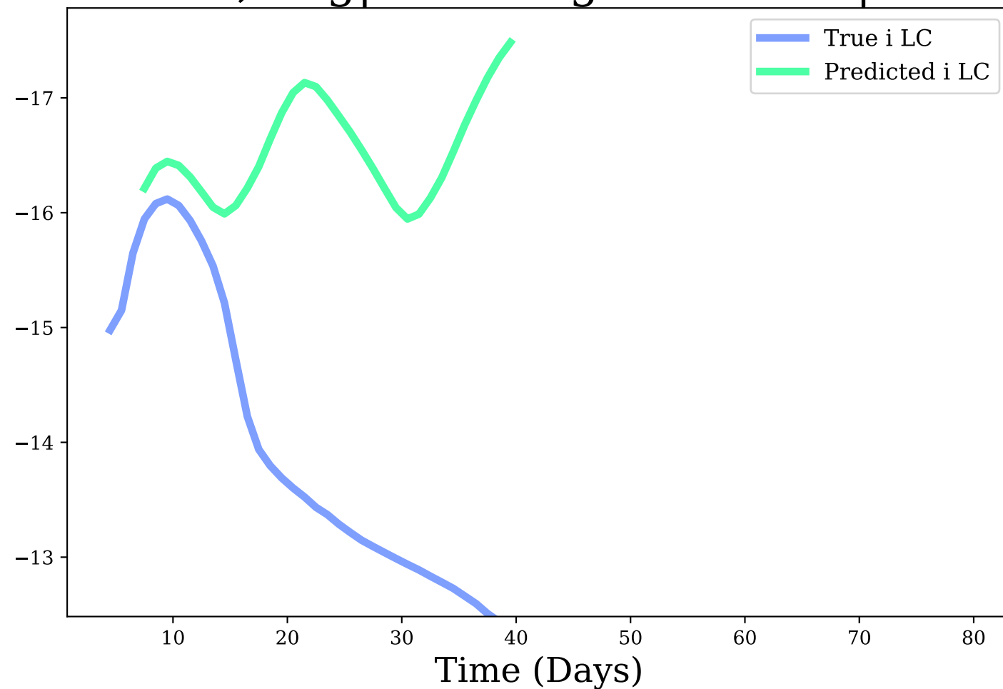
i-band, Avg|Max Mag Diff: 2.71 | 5.13
