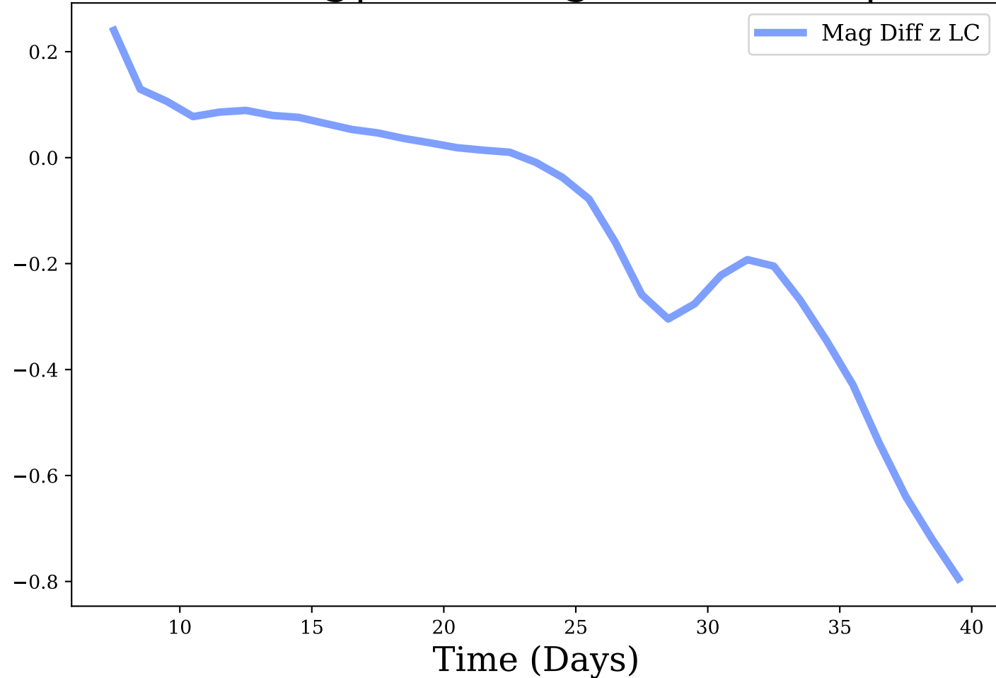
z-band, Avg|Max Mag Diff: -0.13 | 0.79
