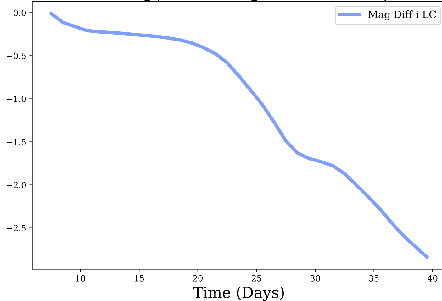
i-band, Avg|Max Mag Diff: -1.08 | 2.84
