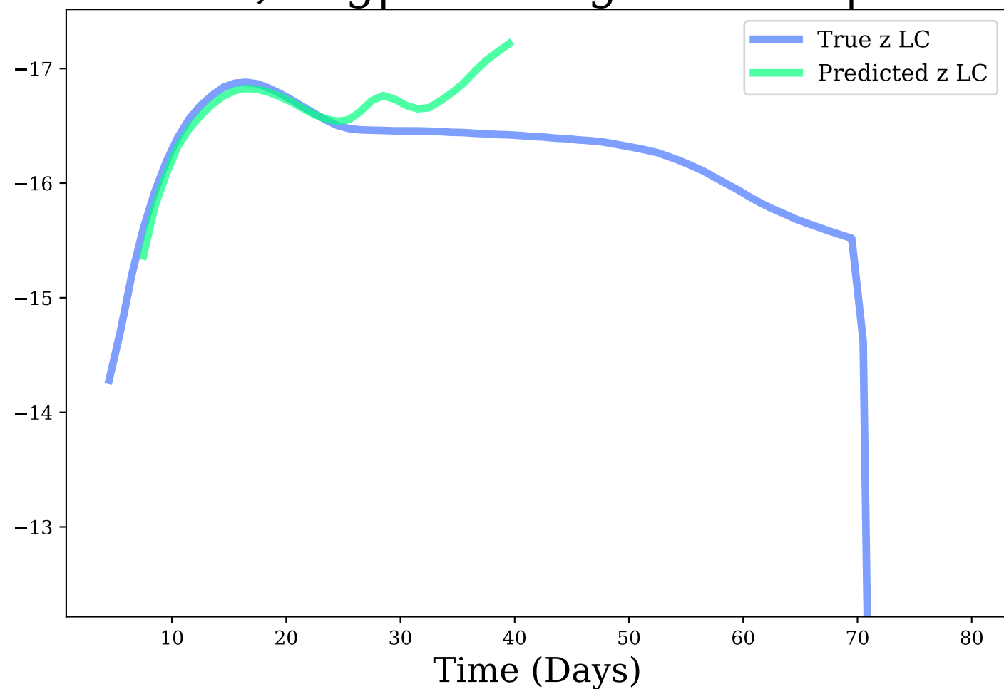
z-band, Avg|Max Mag Diff: 0.2 | 0.79
