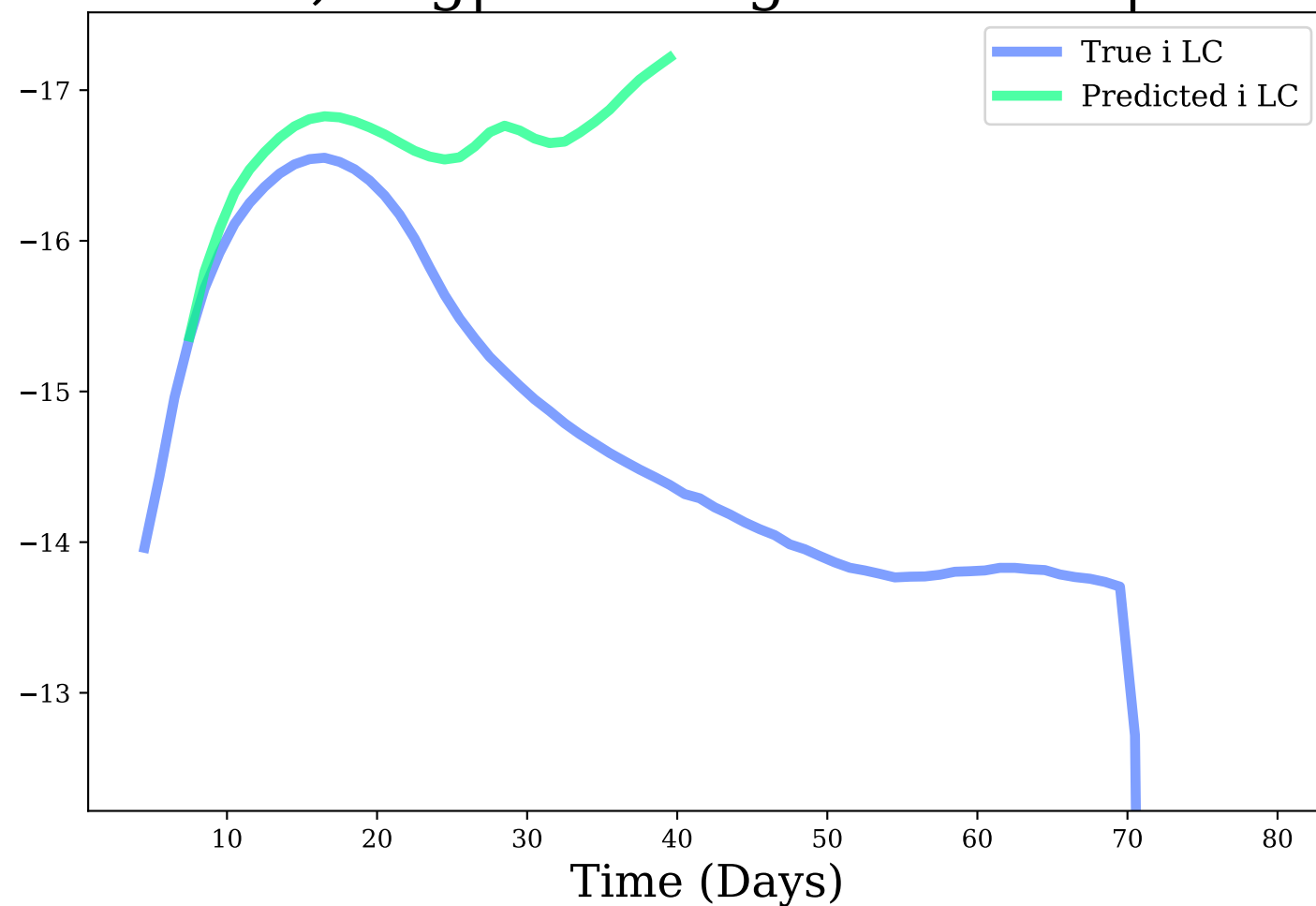
i-band, Avg|Max Mag Diff: 1.08 | 2.84
