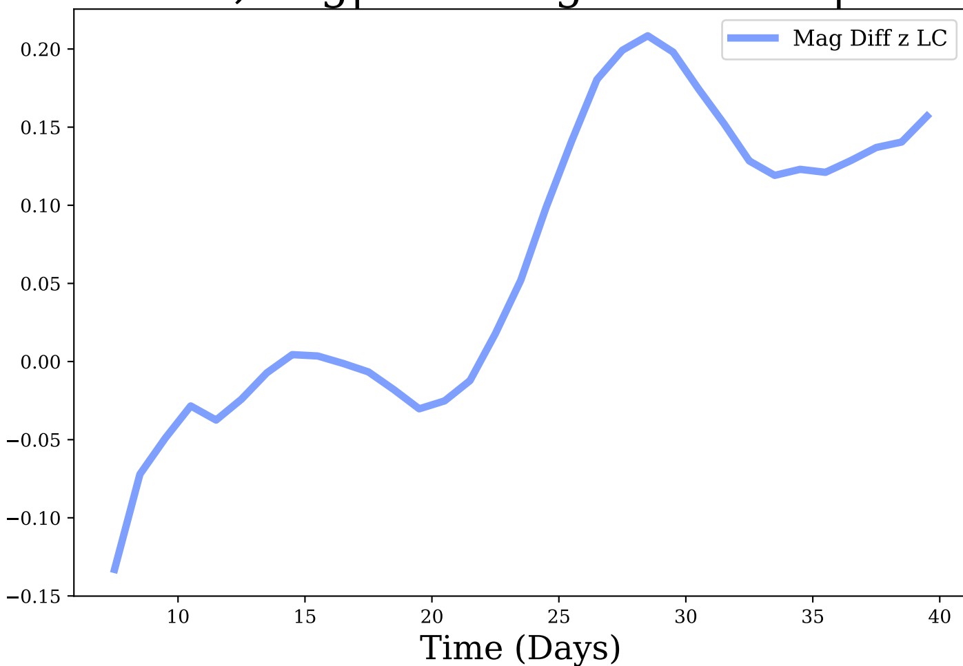
z-band, Avg|Max Mag Diff: 0.06 | 0.21
