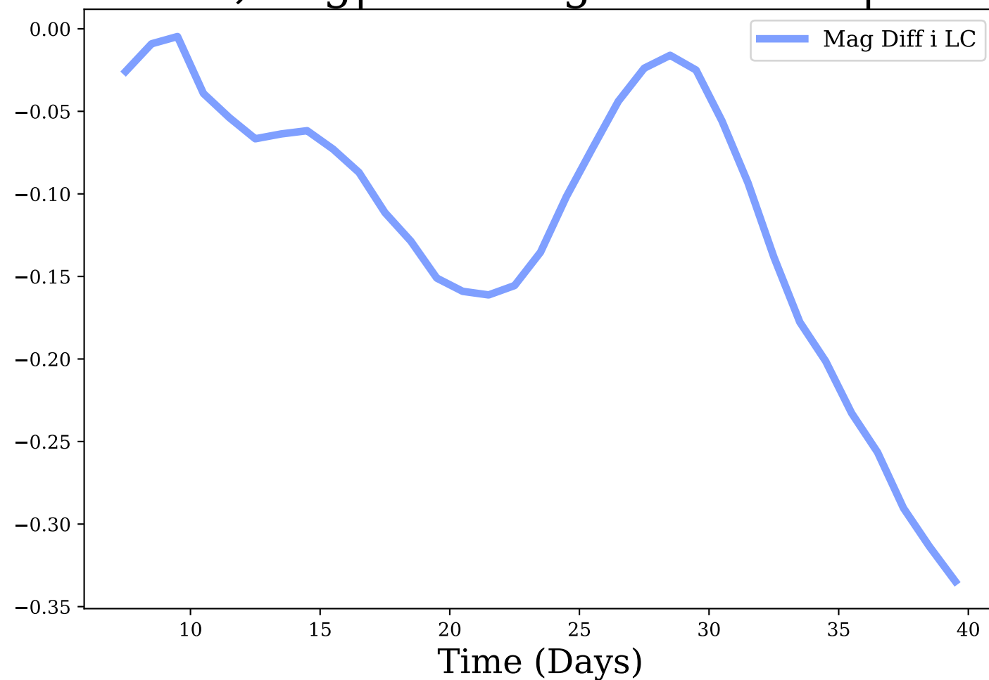
i-band, Avg|Max Mag Diff: -0.12 | 0.33
