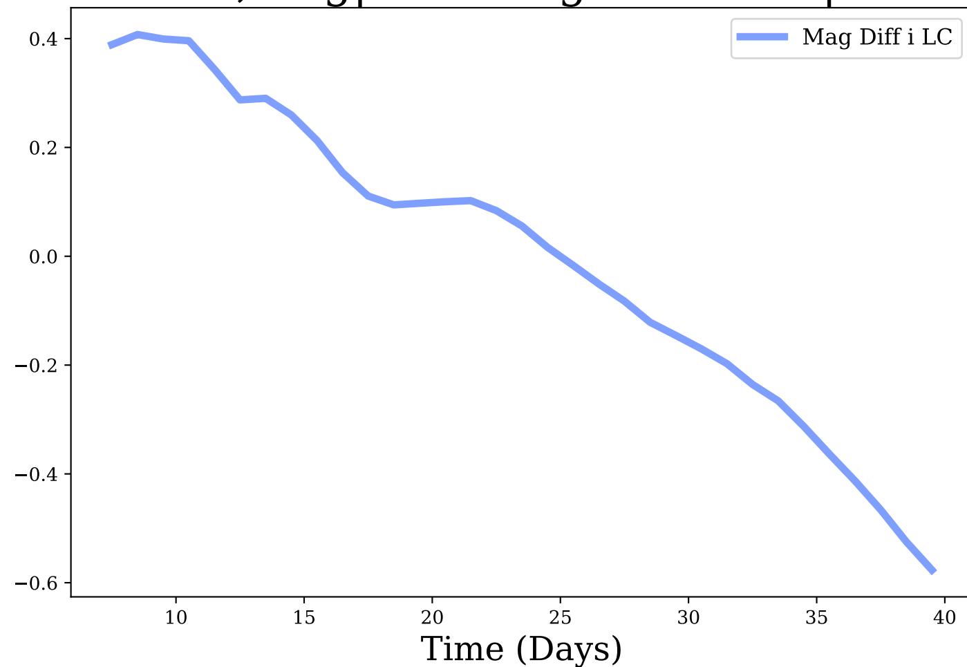
i-band, Avg|Max Mag Diff: -0.0 | 0.58
