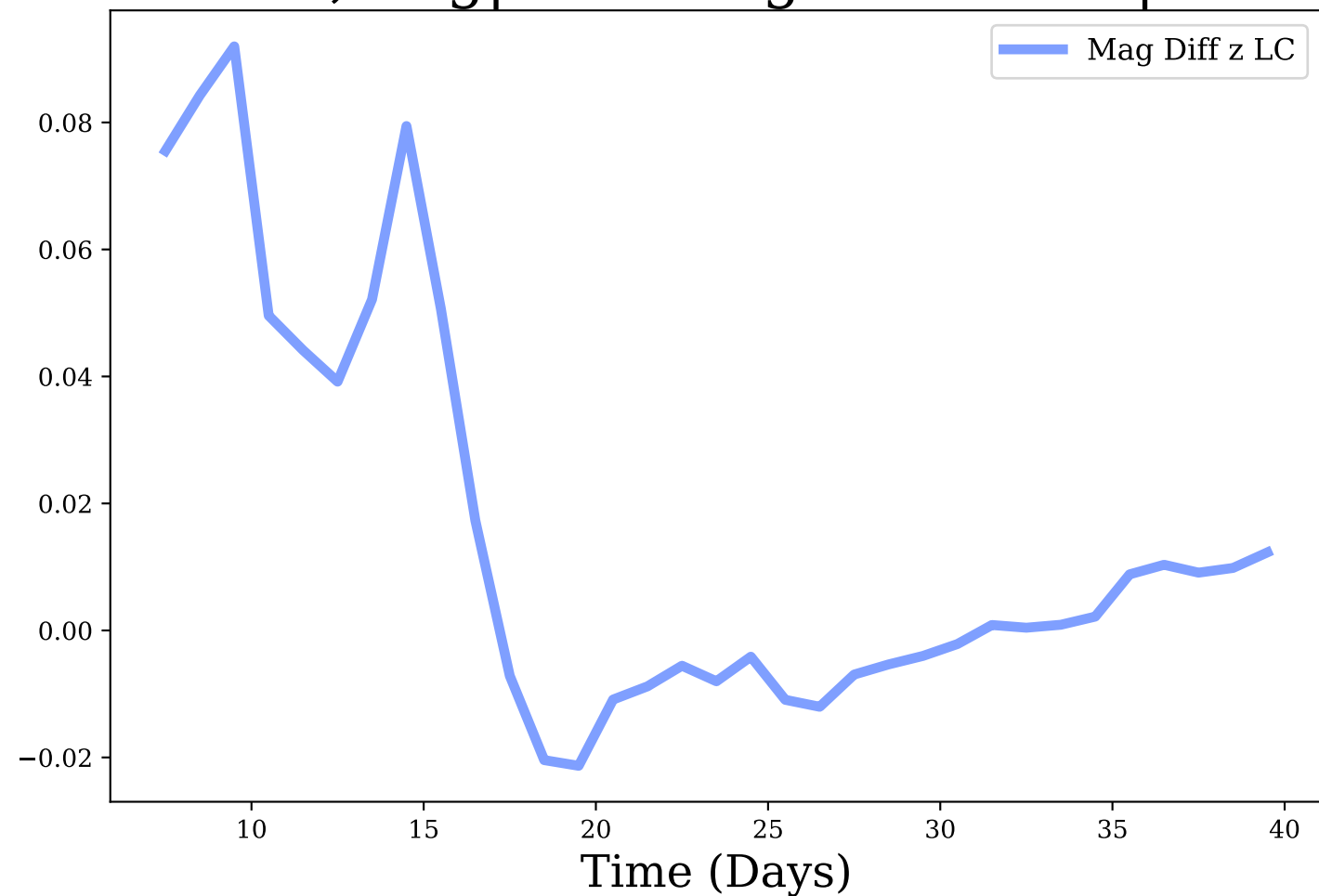
z-band, Avg|Max Mag Diff: 0.02 | 0.09
