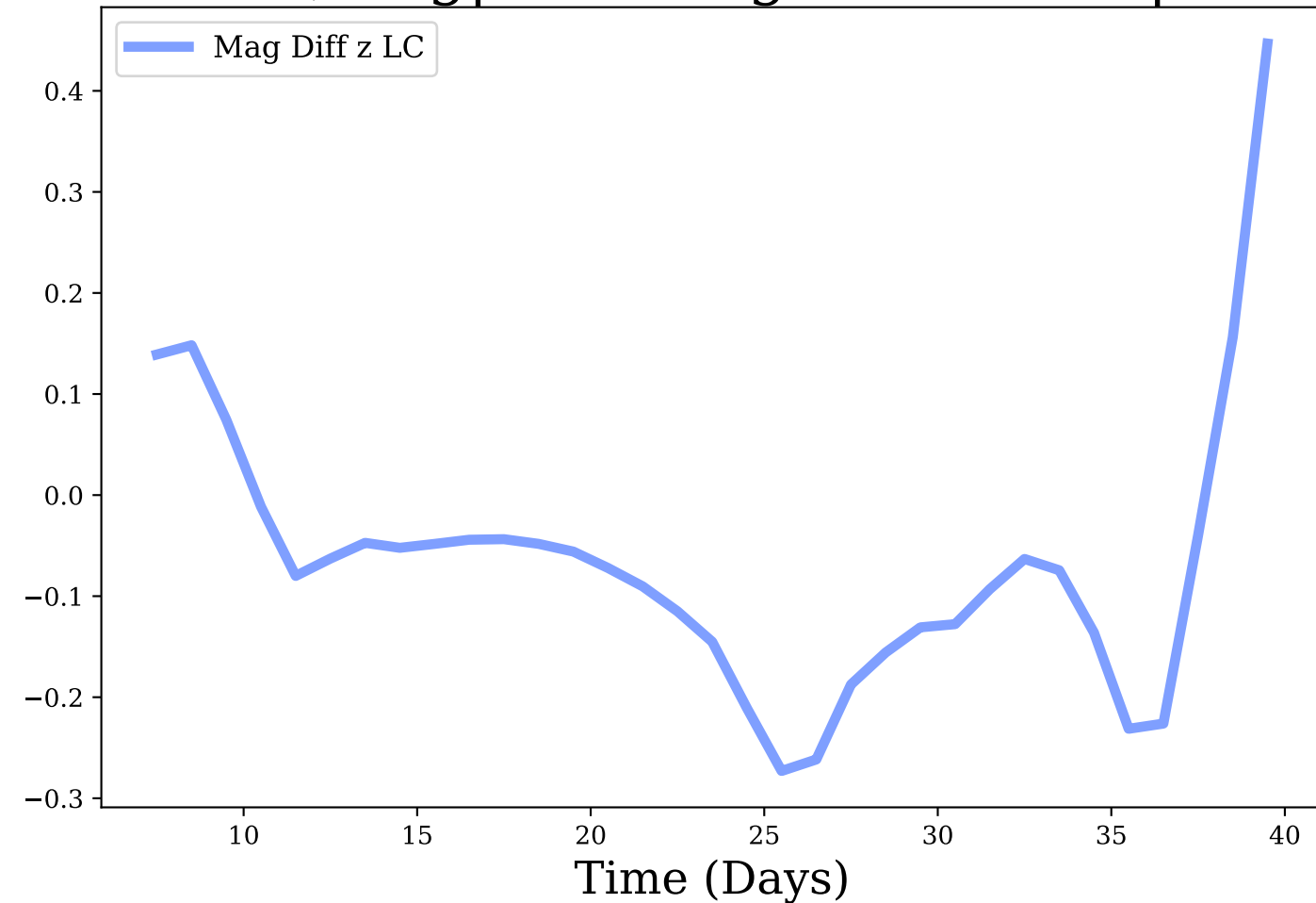
z-band, Avg|Max Mag Diff: -0.07 | 0.45
