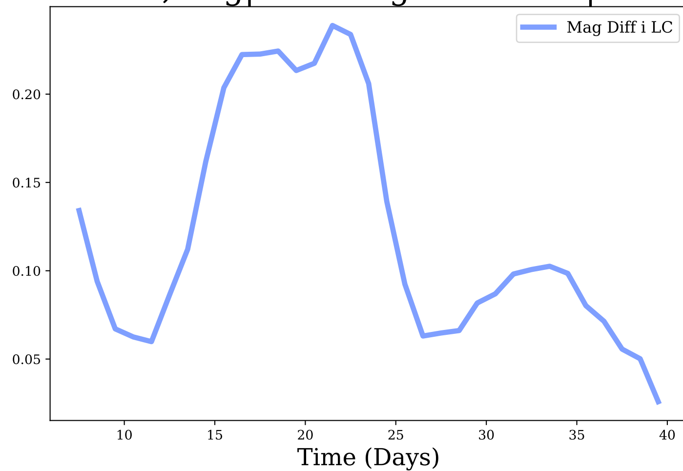
i-band, Avg|Max Mag Diff: 0.12 | 0.24
