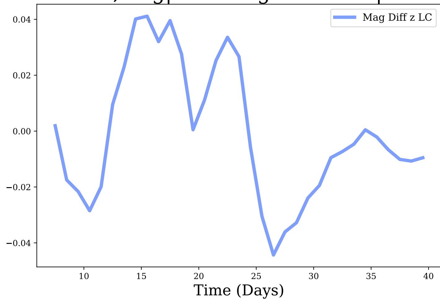
z-band, Avg|Max Mag Diff: -0.0 | 0.04
