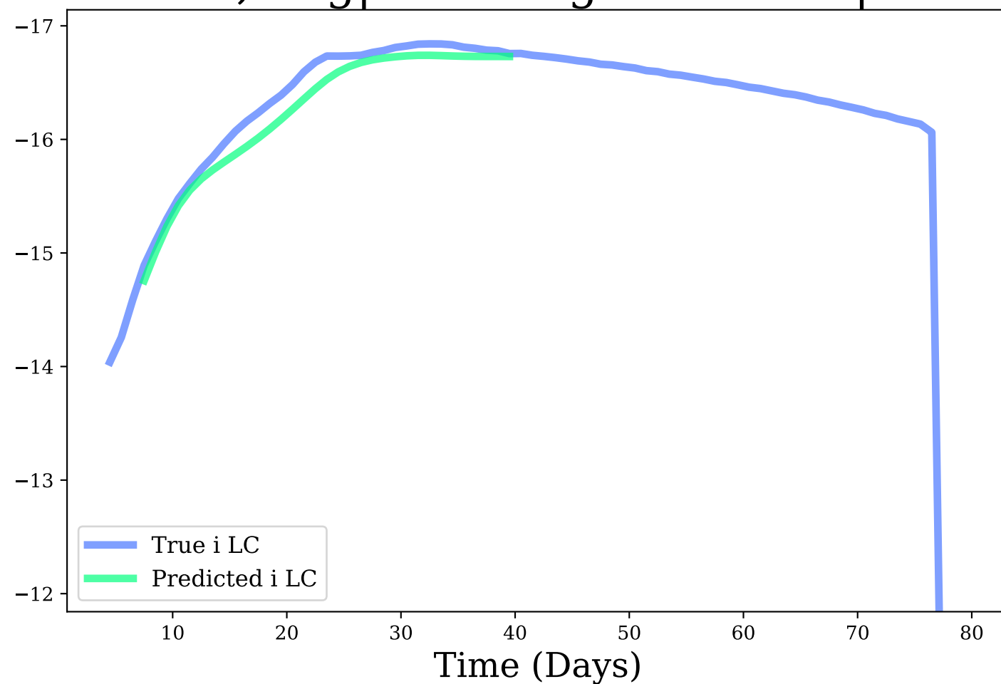
i-band, Avg|Max Mag Diff: 0.12 | 0.24
