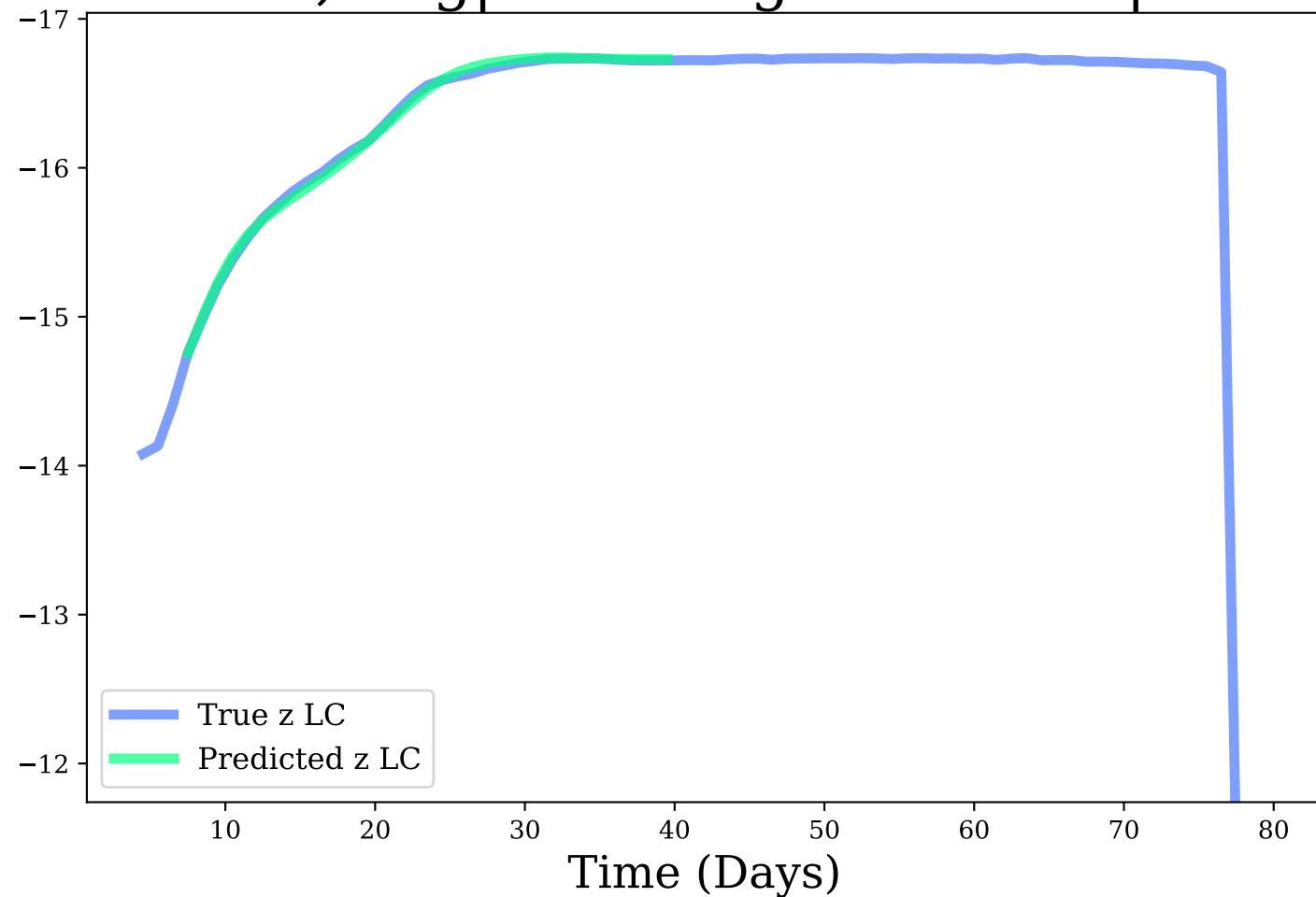
z-band, Avg|Max Mag Diff: 0.02 | 0.04
