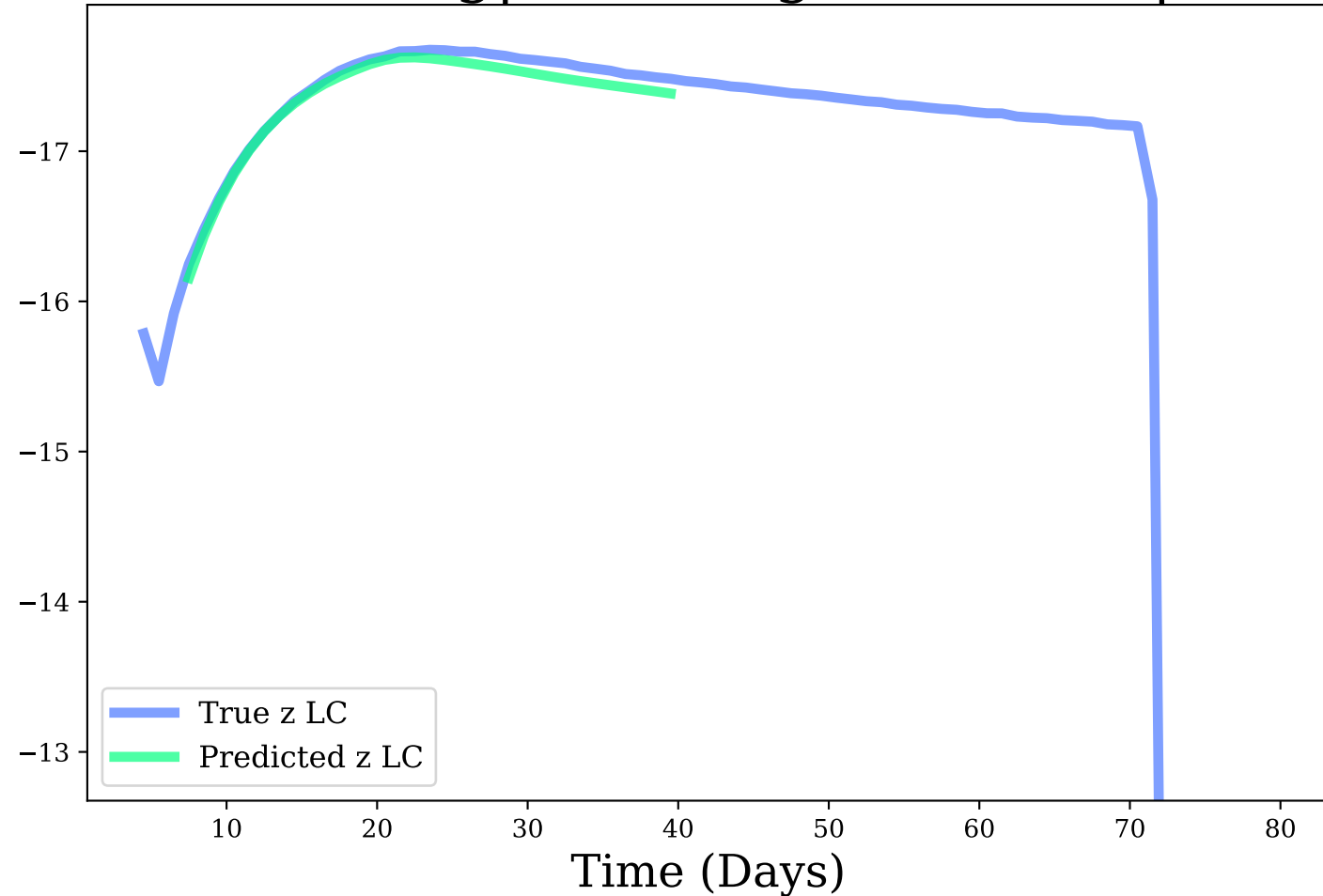
z-band, Avg|Max Mag Diff: 0.06 | 0.1
