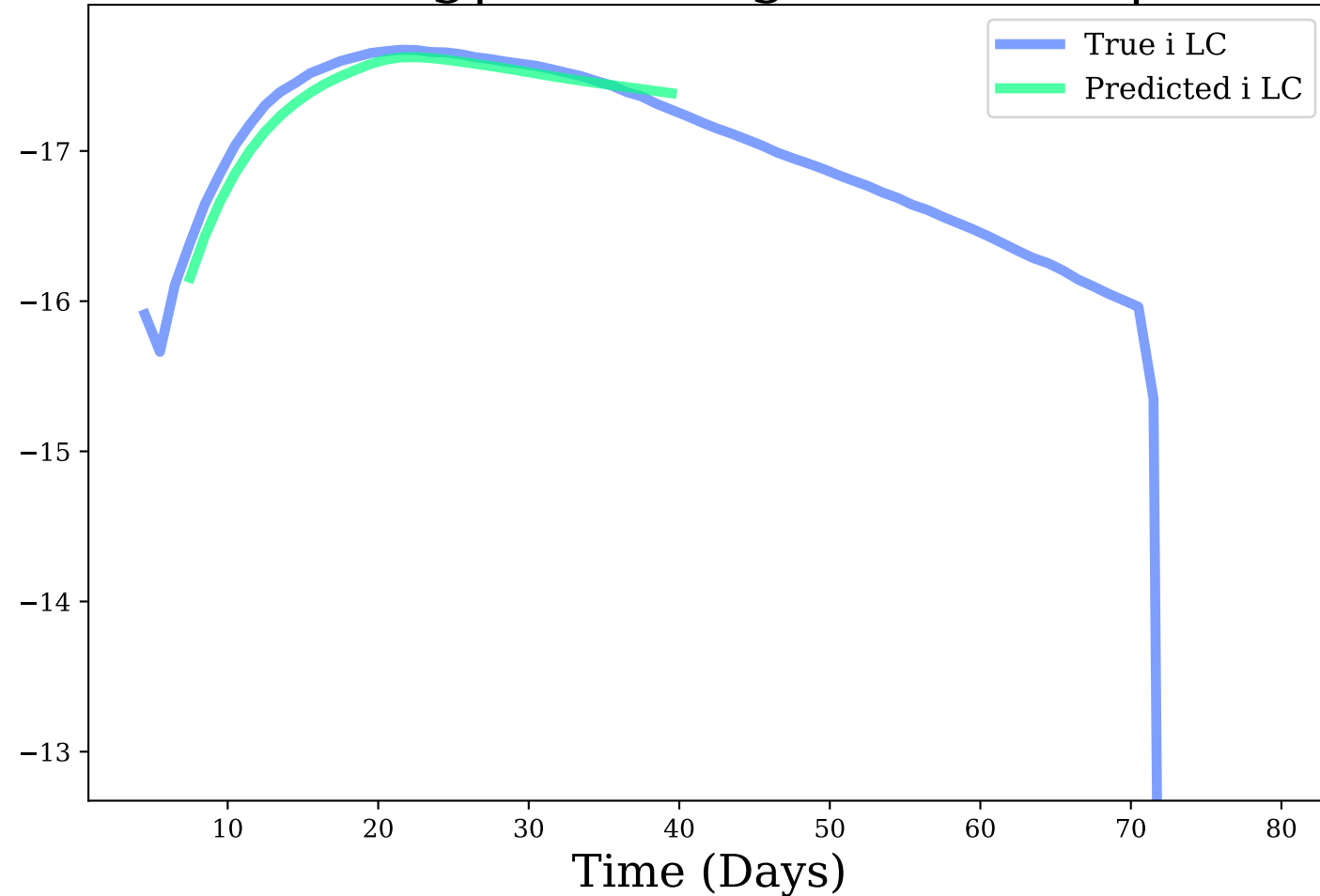
i-band, Avg|Max Mag Diff: 0.09 | 0.23
