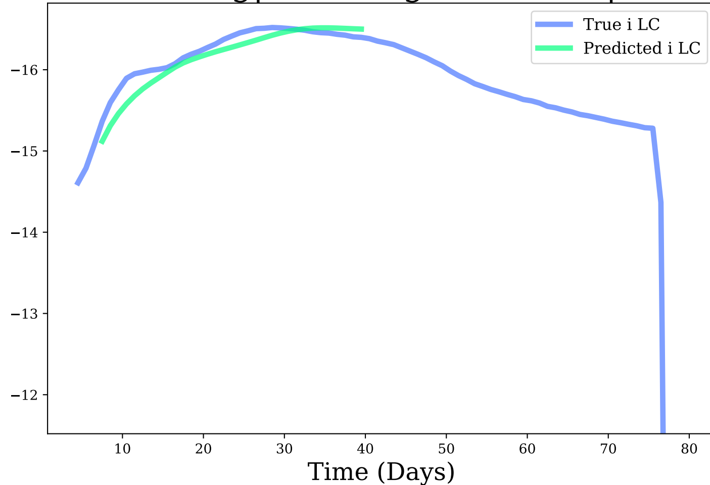
i-band, Avg|Max Mag Diff: 0.12 | 0.32
