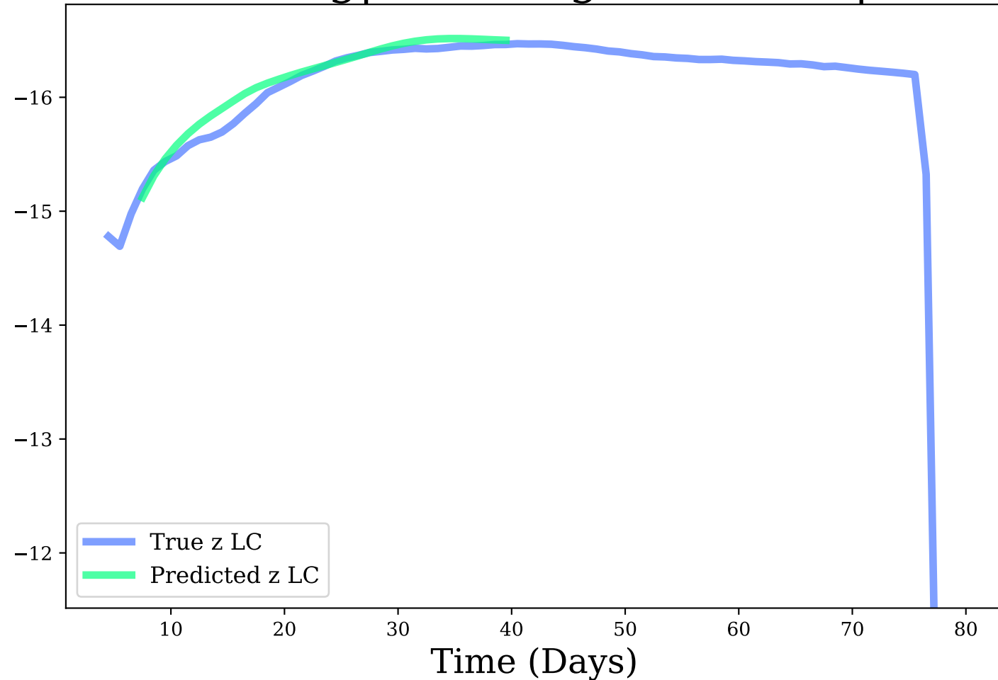
z-band, Avg|Max Mag Diff: 0.07 | 0.21
