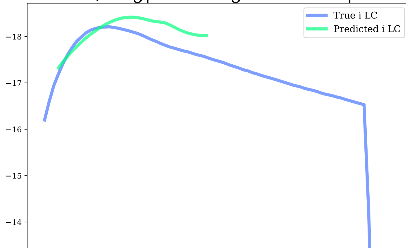
i-band, Avg|Max Mag Diff: 0.27 | 0.48
