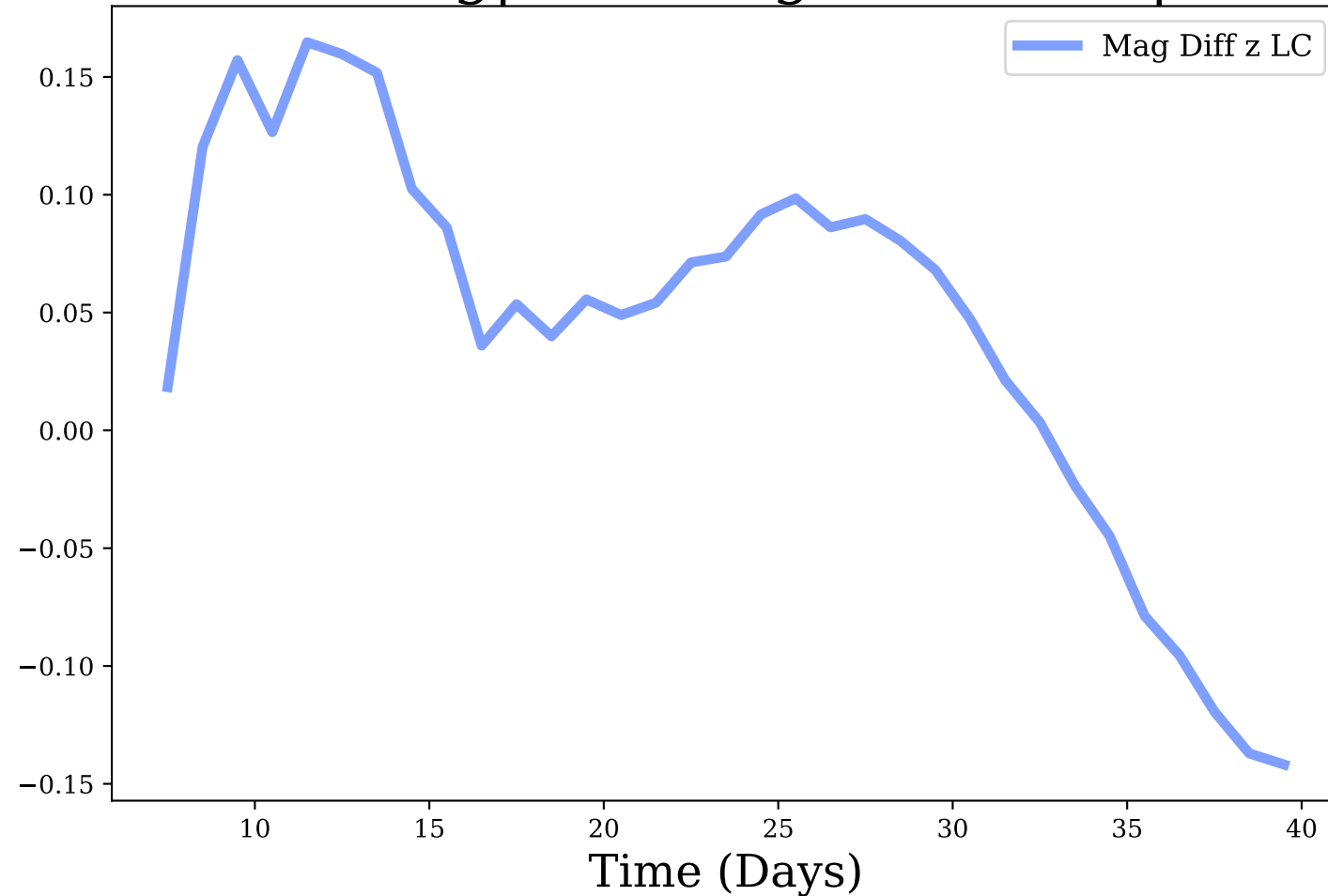
z-band, Avg|Max Mag Diff: 0.04 | 0.16
