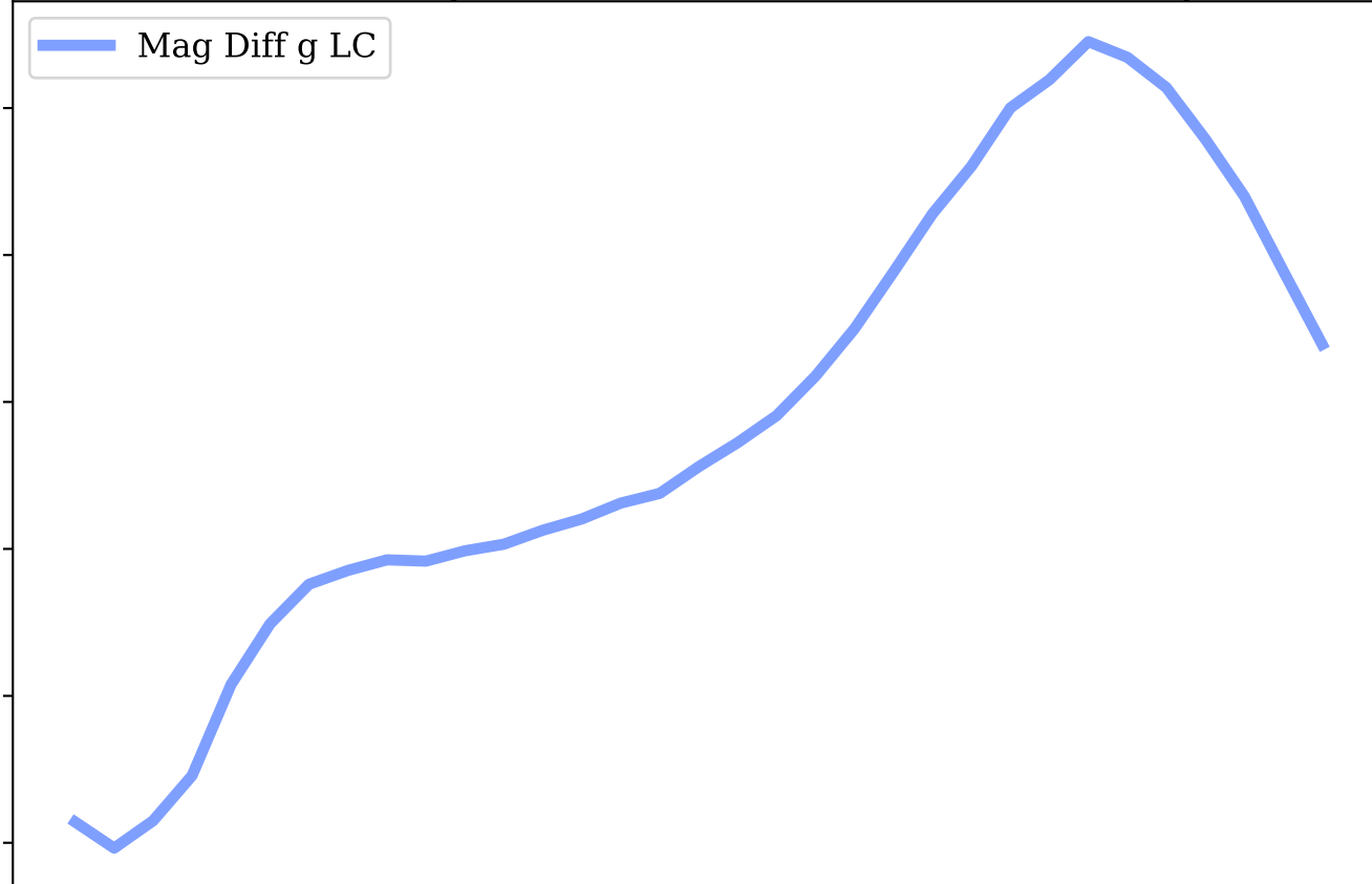
g-band, Avg|Max Mag Diff: 0.78 | 1.05
