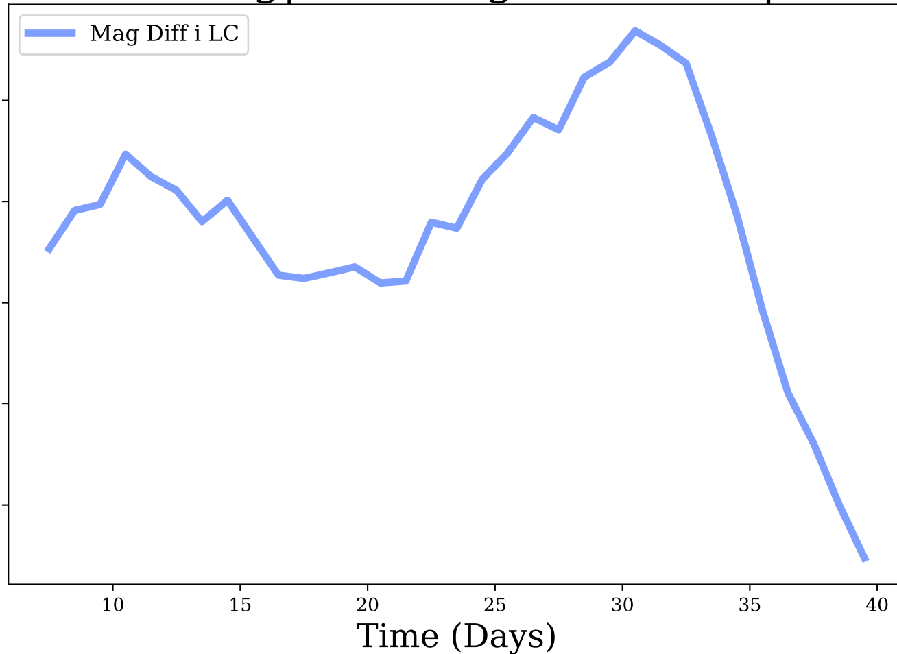
i-band, Avg|Max Mag Diff: 0.24 | 0.33
